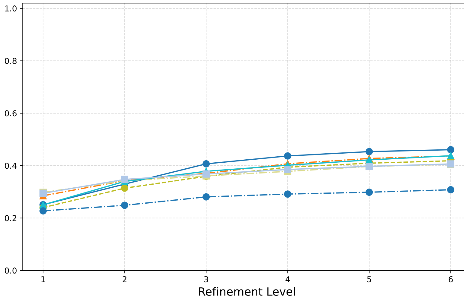
1-form Hodge Laplacian: V-Cycle (Barycentric) - n_{\text{ev}} -largest EV (mag.)
