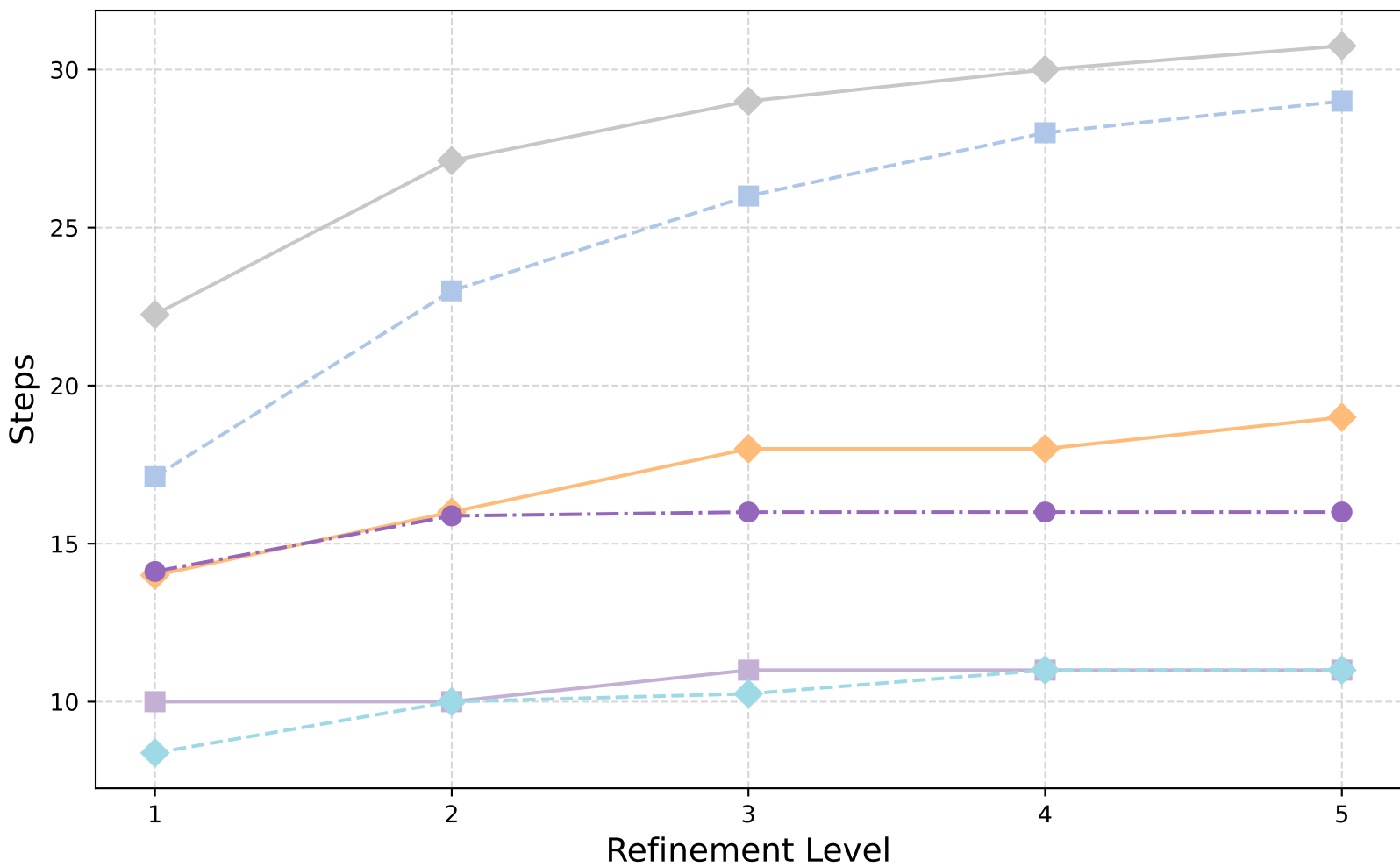
1-form Hodge Laplacian: V-Cycle (Barycentric) - GMRES Iterations
