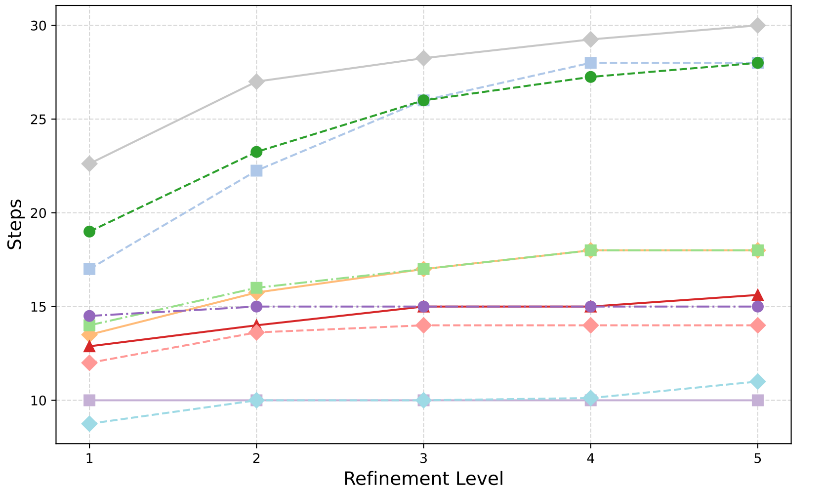
Magnetostatics: W-Cycle (Barycentric) - GMRES Iterations
