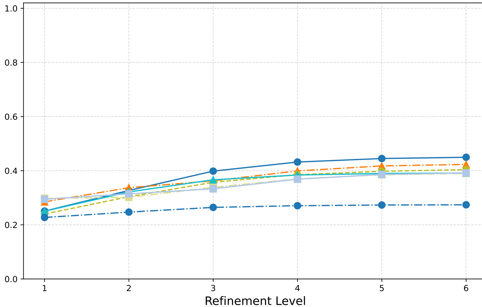
1-form Hodge Laplacian: W-Cycle (Barycentric) - n_{\text{ev}} -largest EV (mag.)
