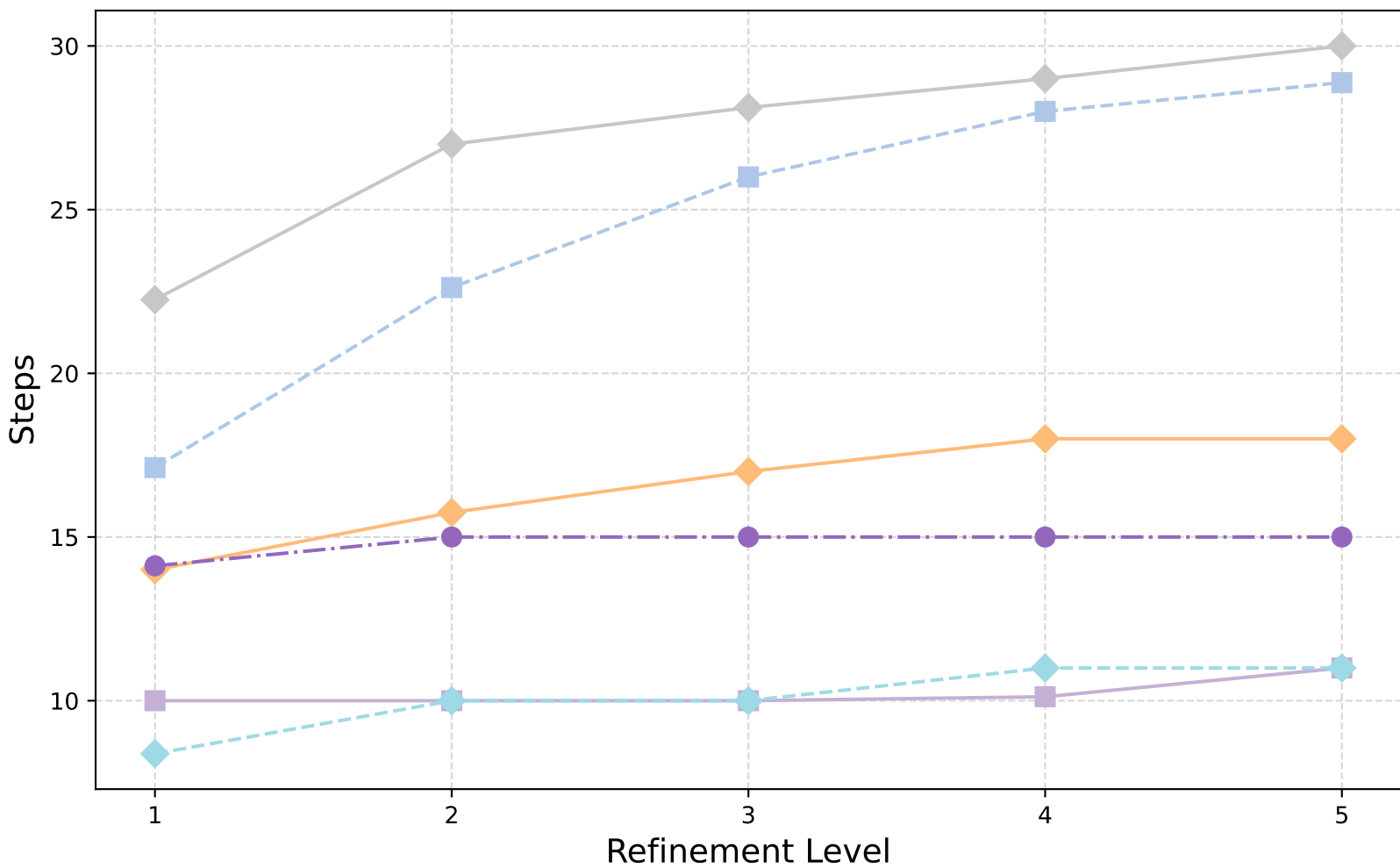
1-form Hodge Laplacian: W-Cycle (Barycentric) - GMRES Iterations
