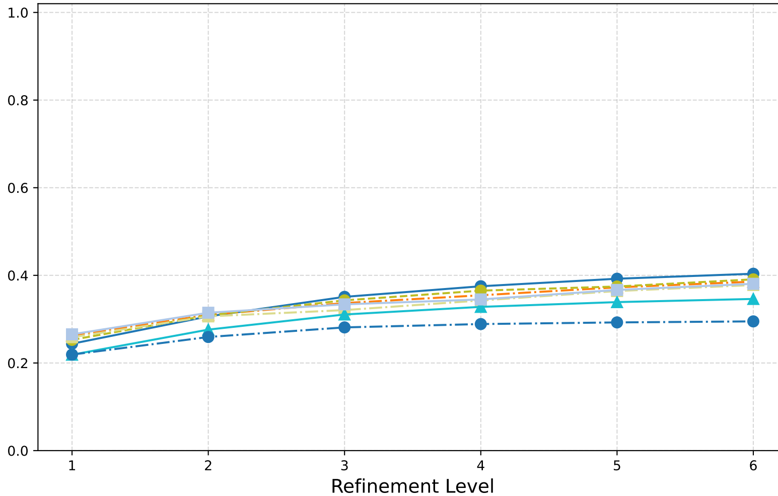
Dirac: V-Cycle (Row Sum) - n_{\text{ev}} -largest EV (mag.)
