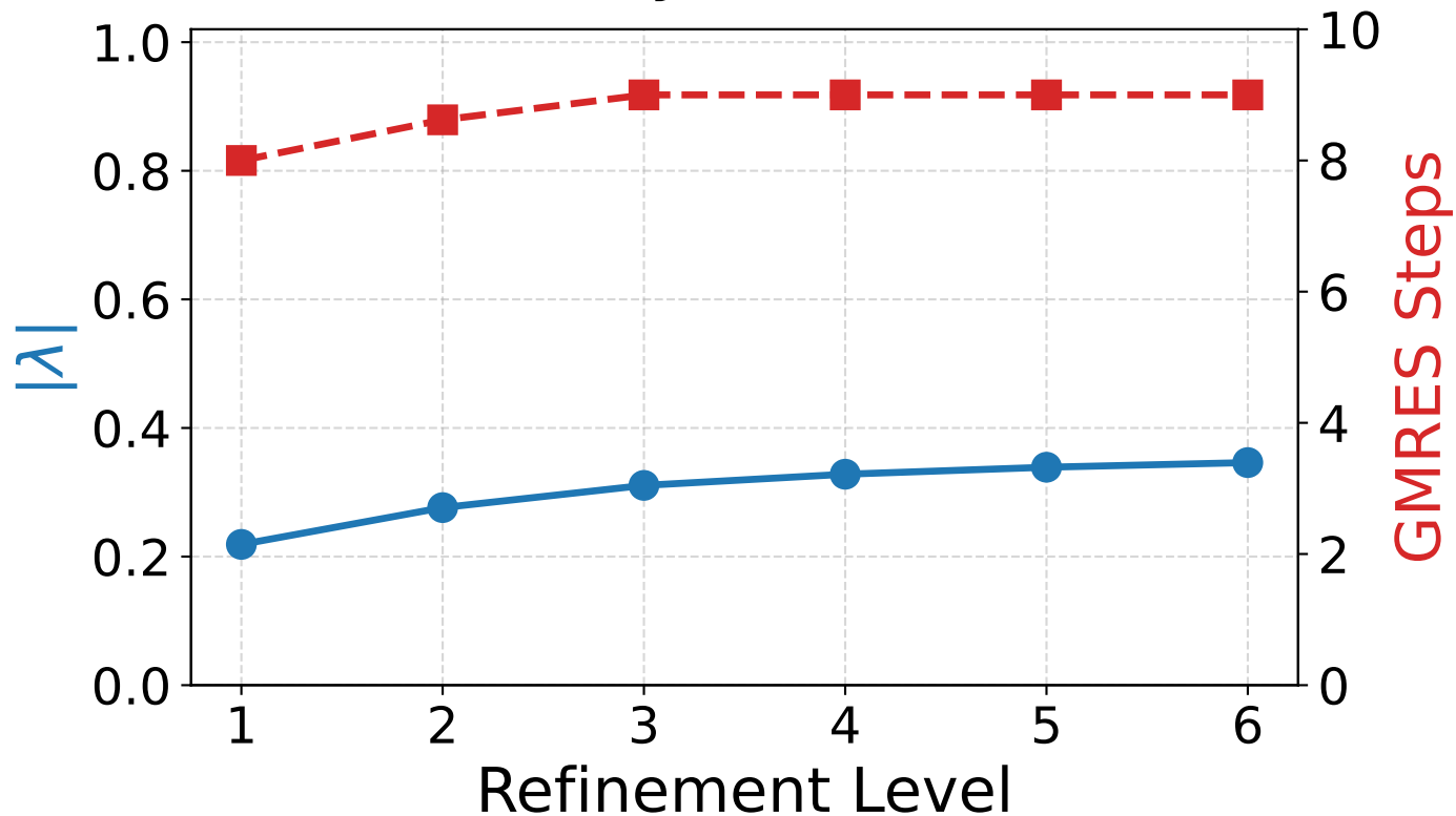
Dirac: V-Cycle (Row Sum)
