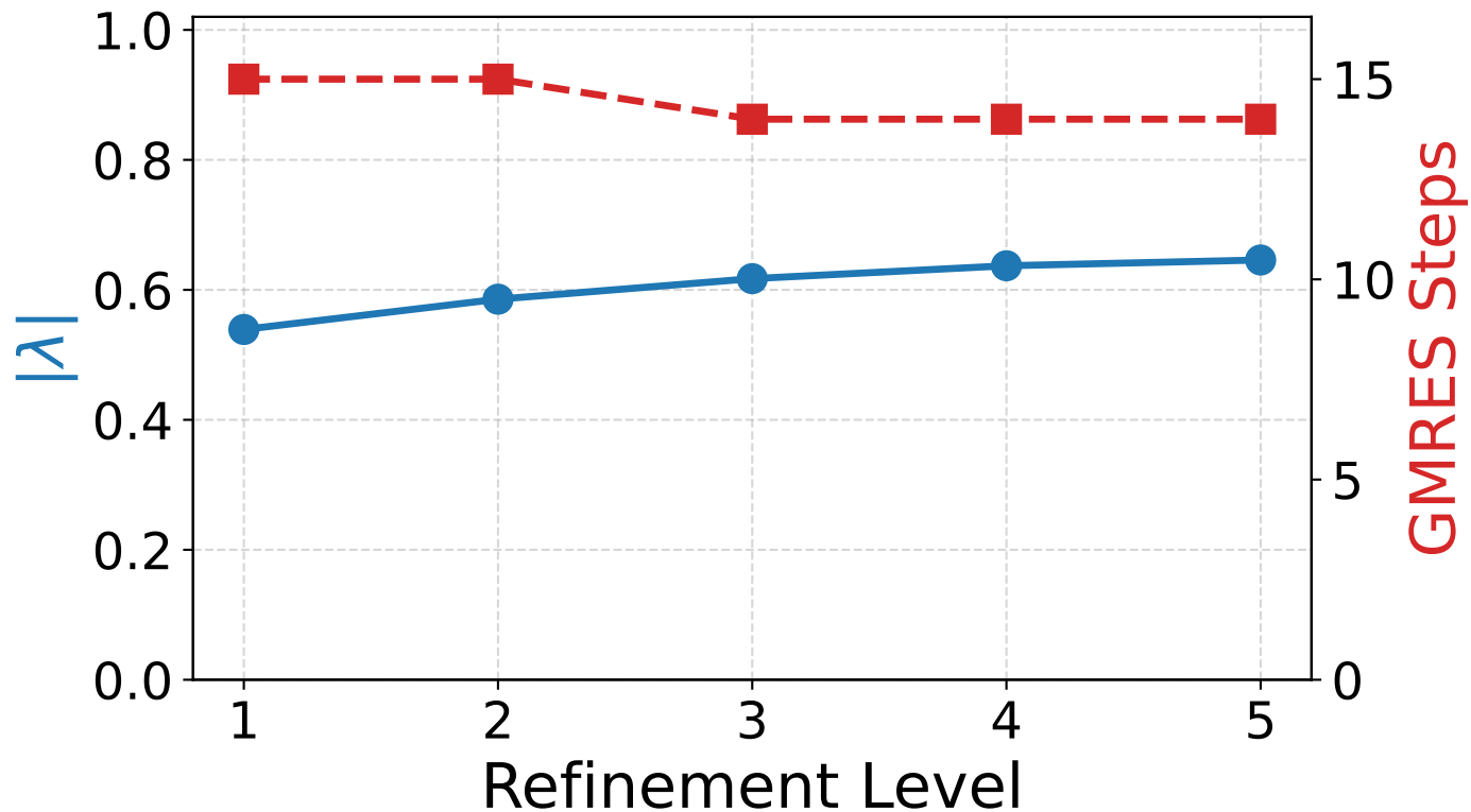
Dirac: V-Cycle (Row Sum)
