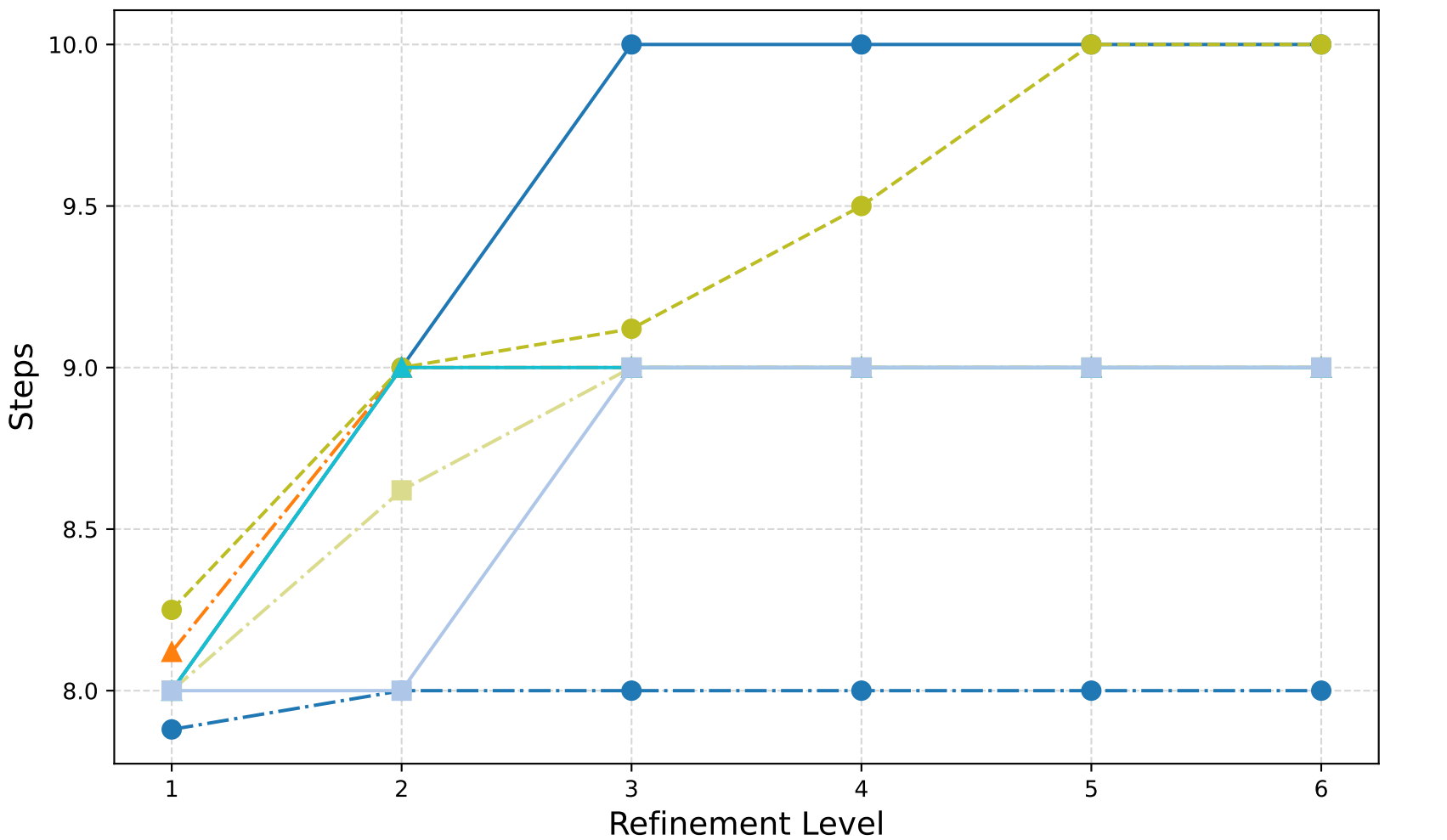
Magnetostatics: V-Cycle (Row Sum) - GMRES Iterations
