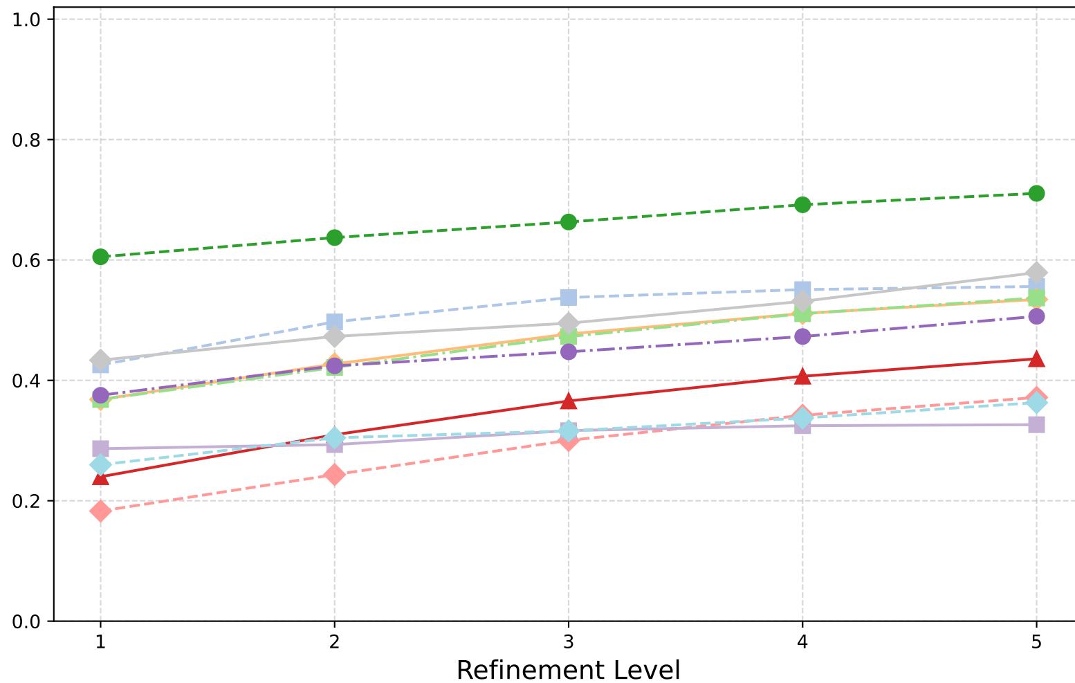
Magnetostatics: V-Cycle (Row Sum) - n_{\text{ev}} -largest EV (mag.)
