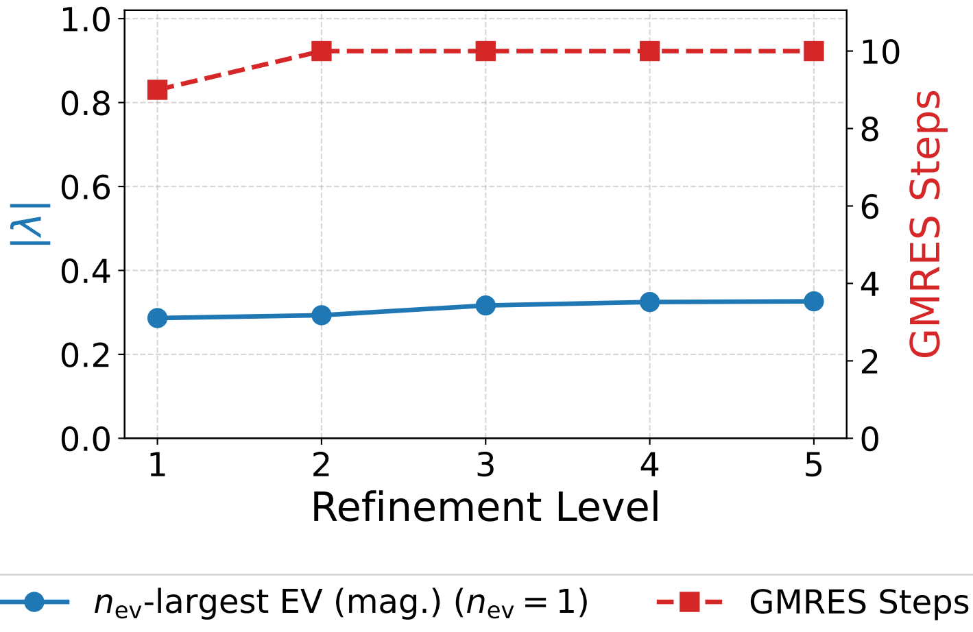
Magnetostatics: V-Cycle (Row Sum)
