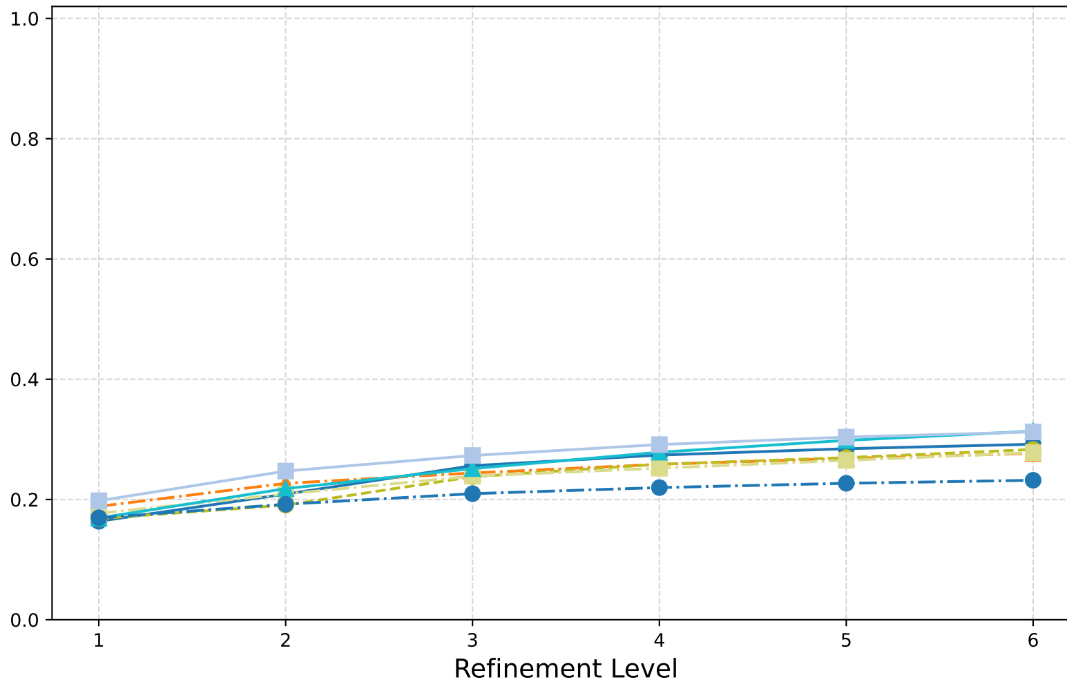
1-form Hodge Laplacian: V-Cycle (Row Sum) - n_{\text{ev}} -largest EV (mag.)
