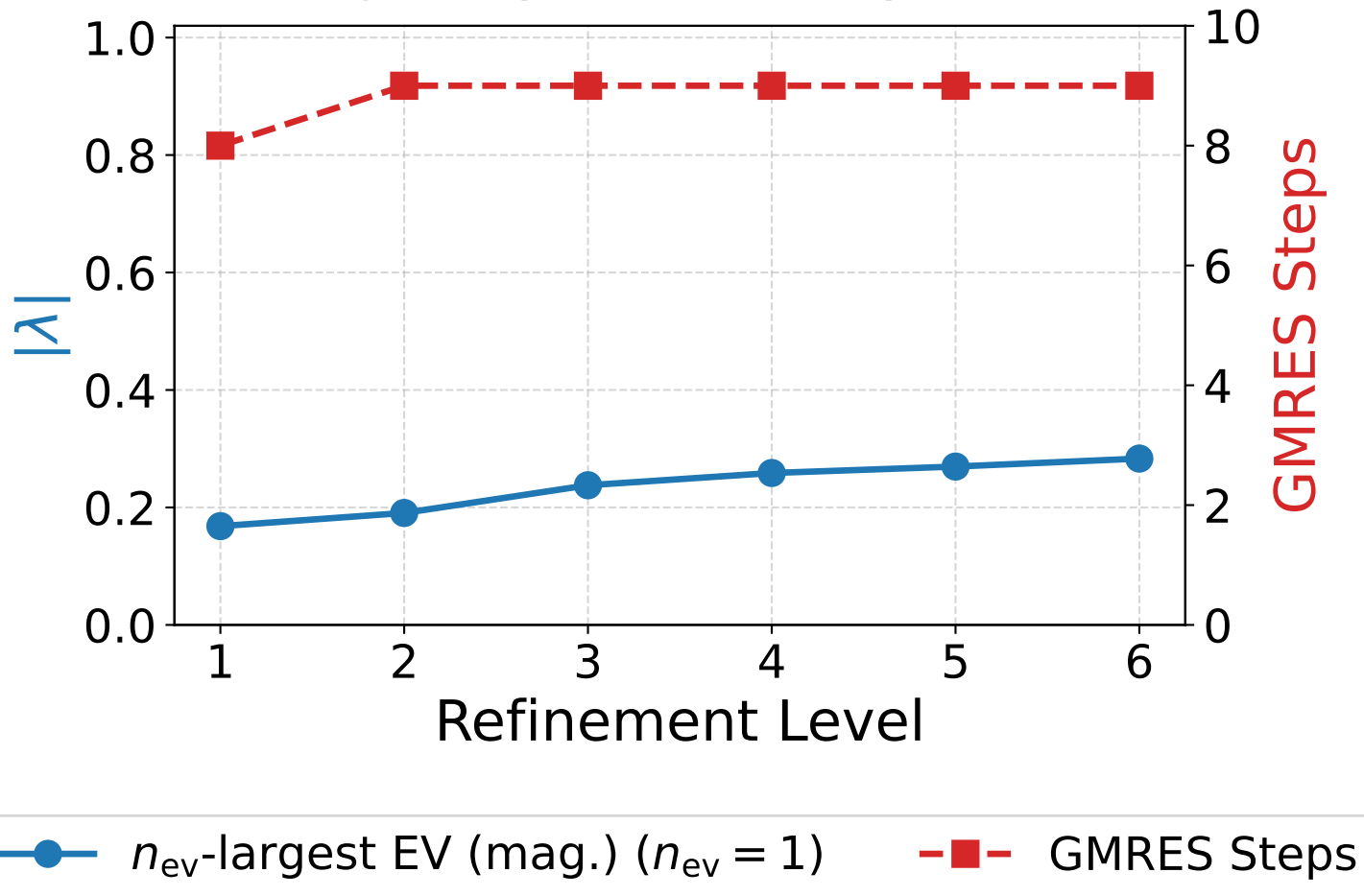
1-form Hodge Laplacian: V-Cycle (Row Sum)
