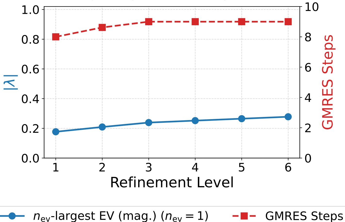
1-form Hodge Laplacian: V-Cycle (Row Sum)
