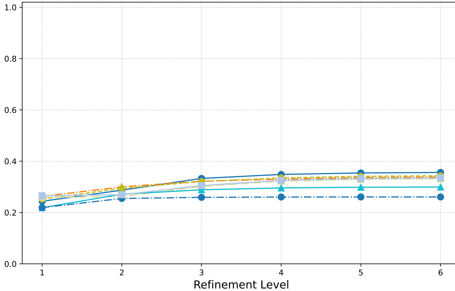
Dirac: W-Cycle (Row Sum) - n_{\text{ev}} -largest EV (mag.)
