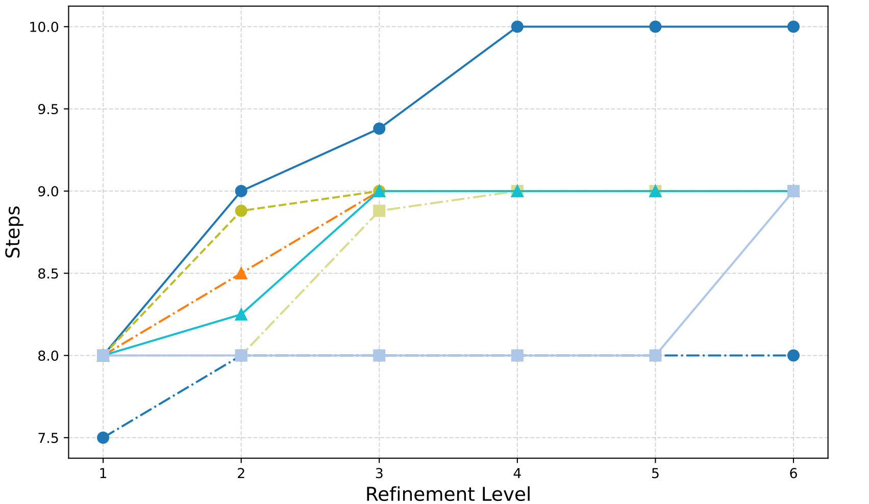
Dirac: W-Cycle (Row Sum) - GMRES Iterations
