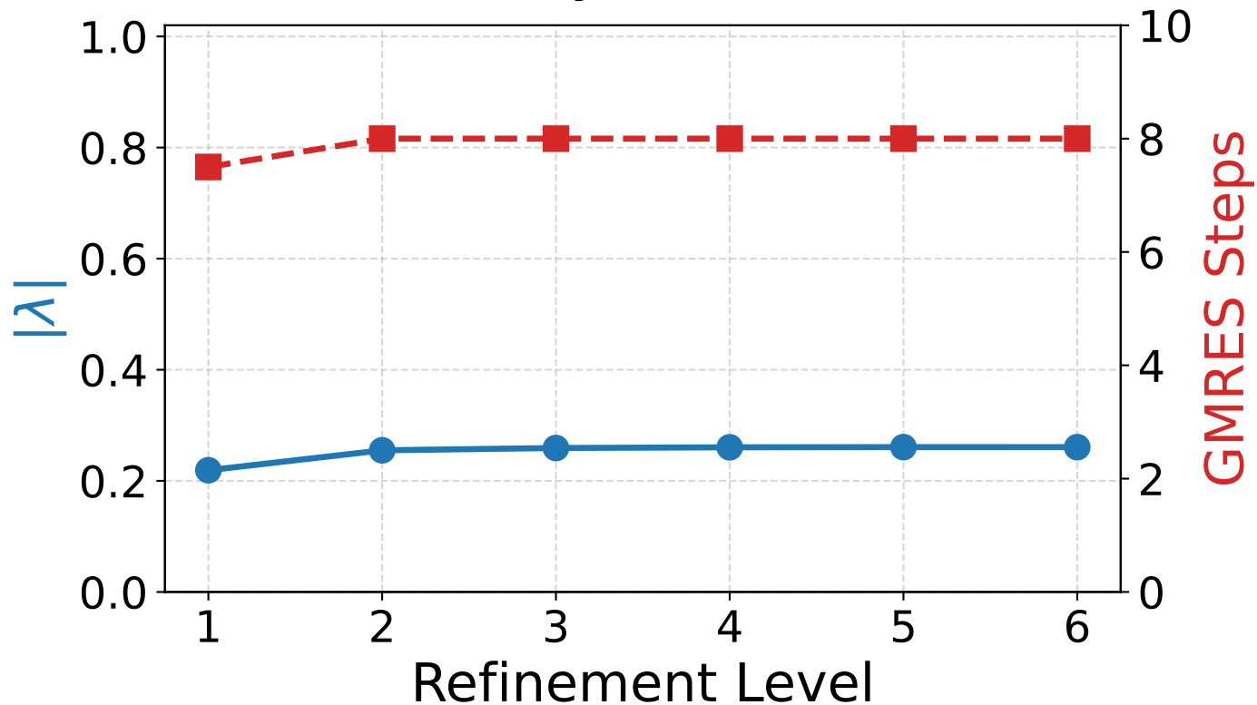
Dirac: W-Cycle (Row Sum)
