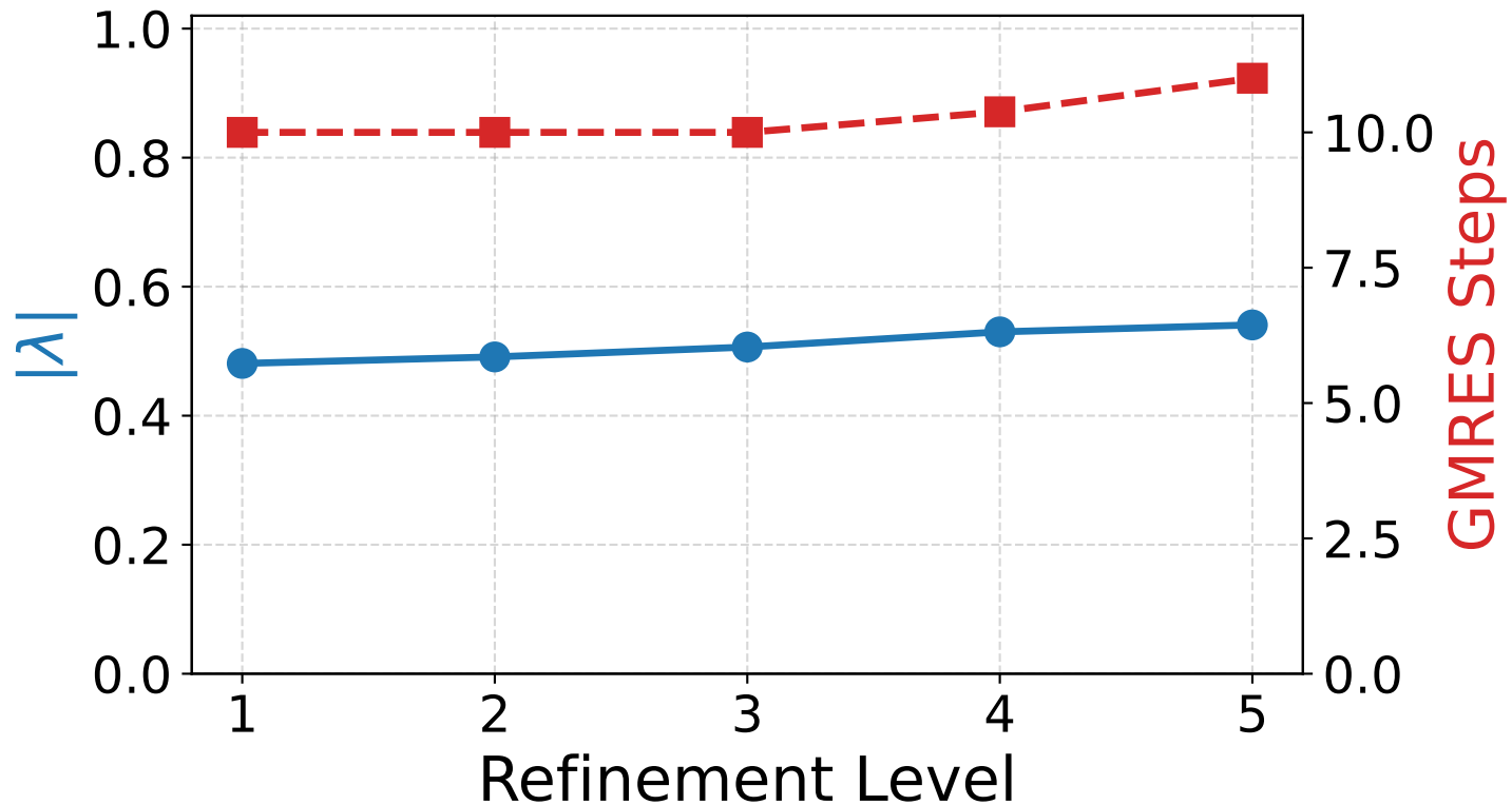
Dirac: W-Cycle (Row Sum)
