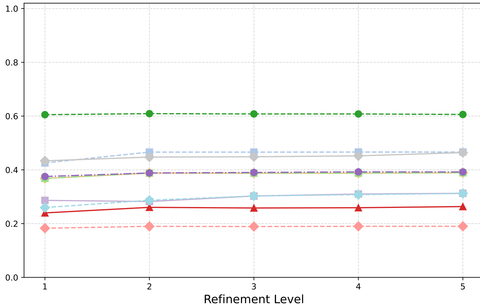
Magnetostatics: W-Cycle (Row Sum) - n_{\text{ev}} -largest EV (mag.)
