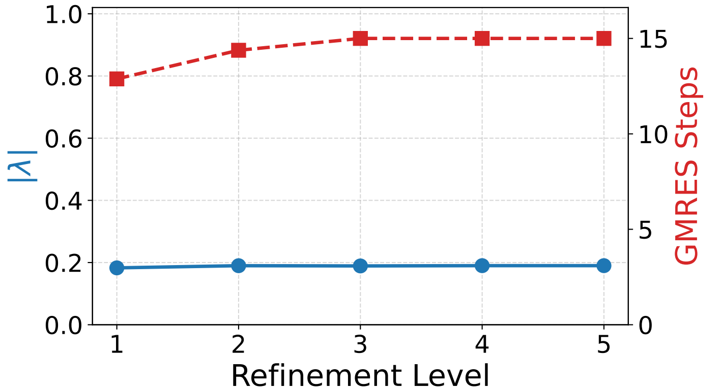
Magnetostatics: W-Cycle (Row Sum)
