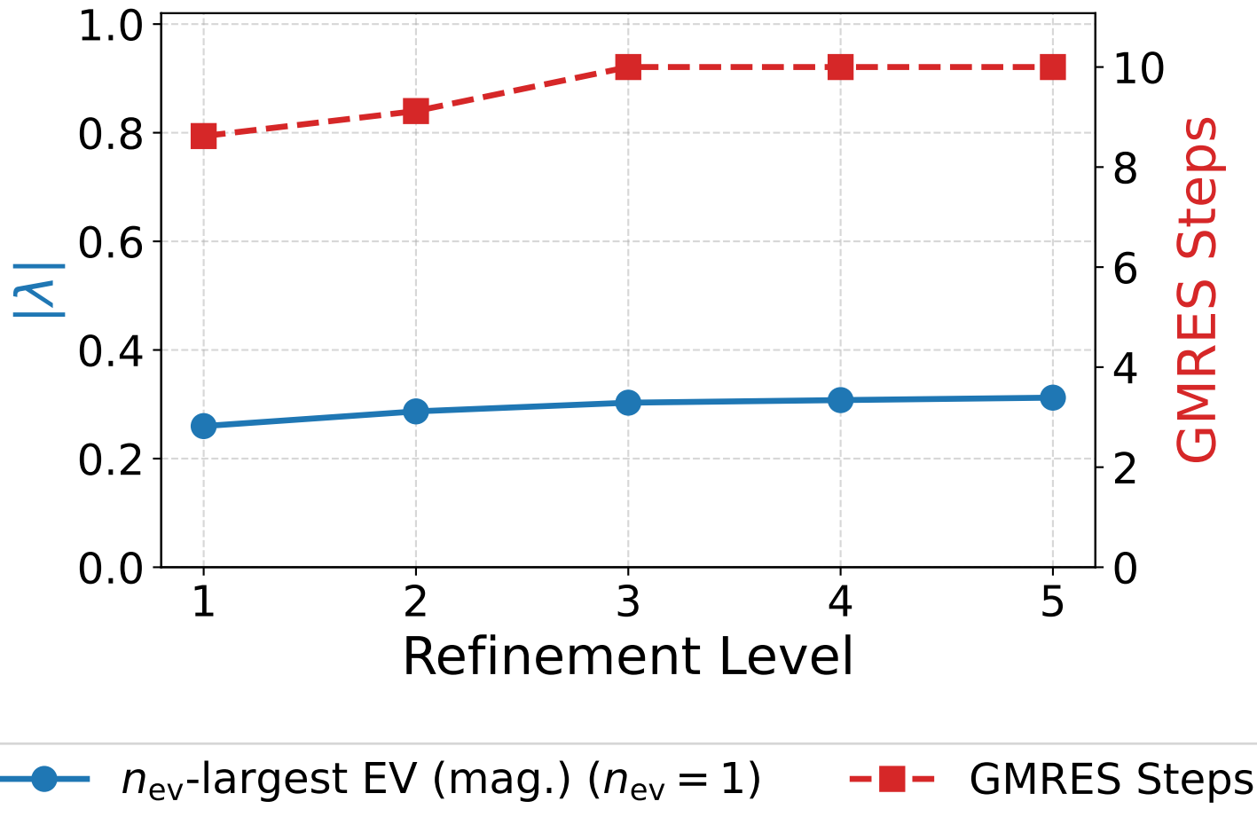
Magnetostatics: W-Cycle (Row Sum)
