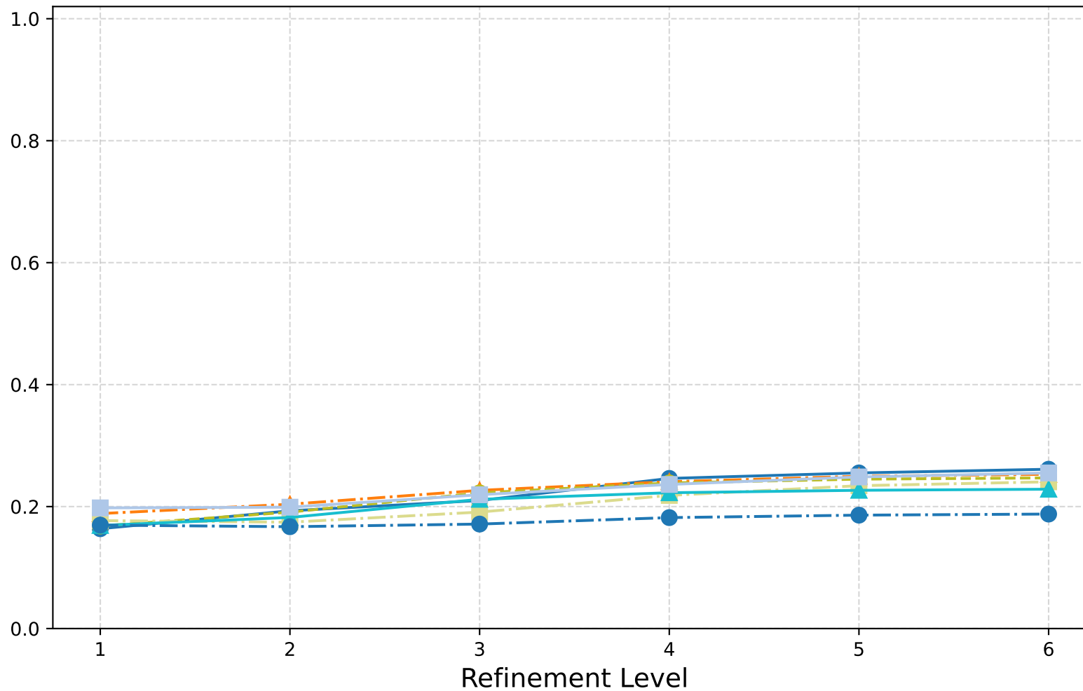
1-form Hodge Laplacian: W-Cycle (Row Sum) - n_{\text{ev}} -largest EV (mag.)
