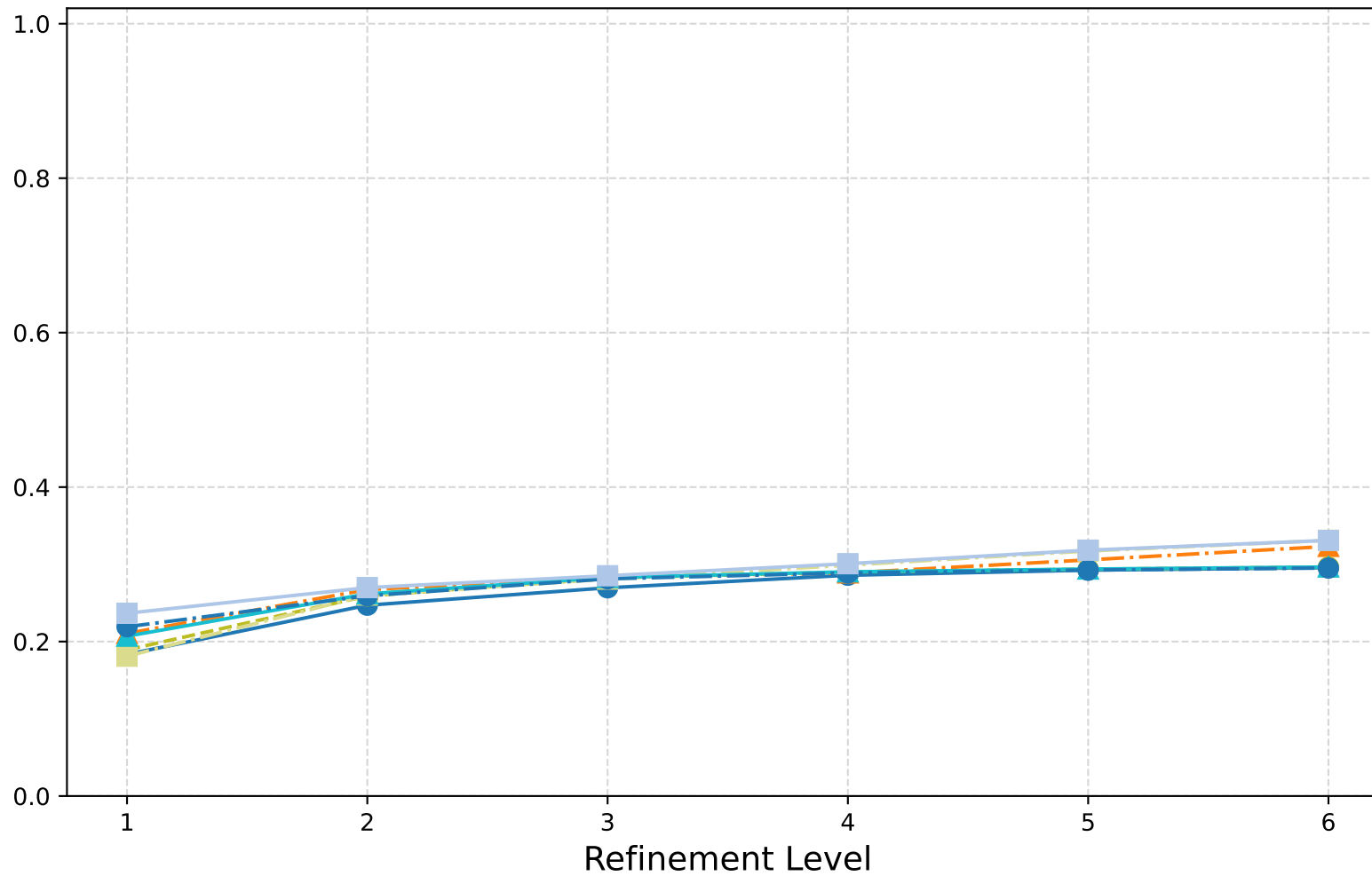
Dirac: V-Cycle (Scaled Id) - n_{\text{ev}} -largest EV (mag.)
