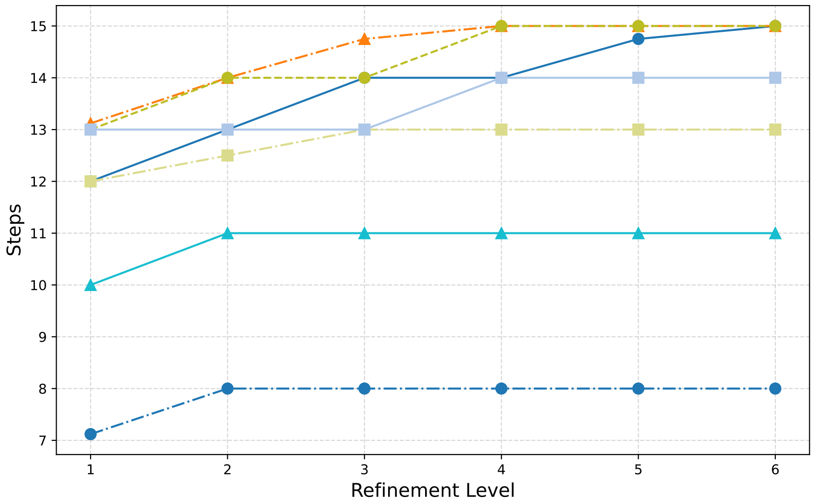
Dirac: V-Cycle (ScaledId) - GMRES Iterations
