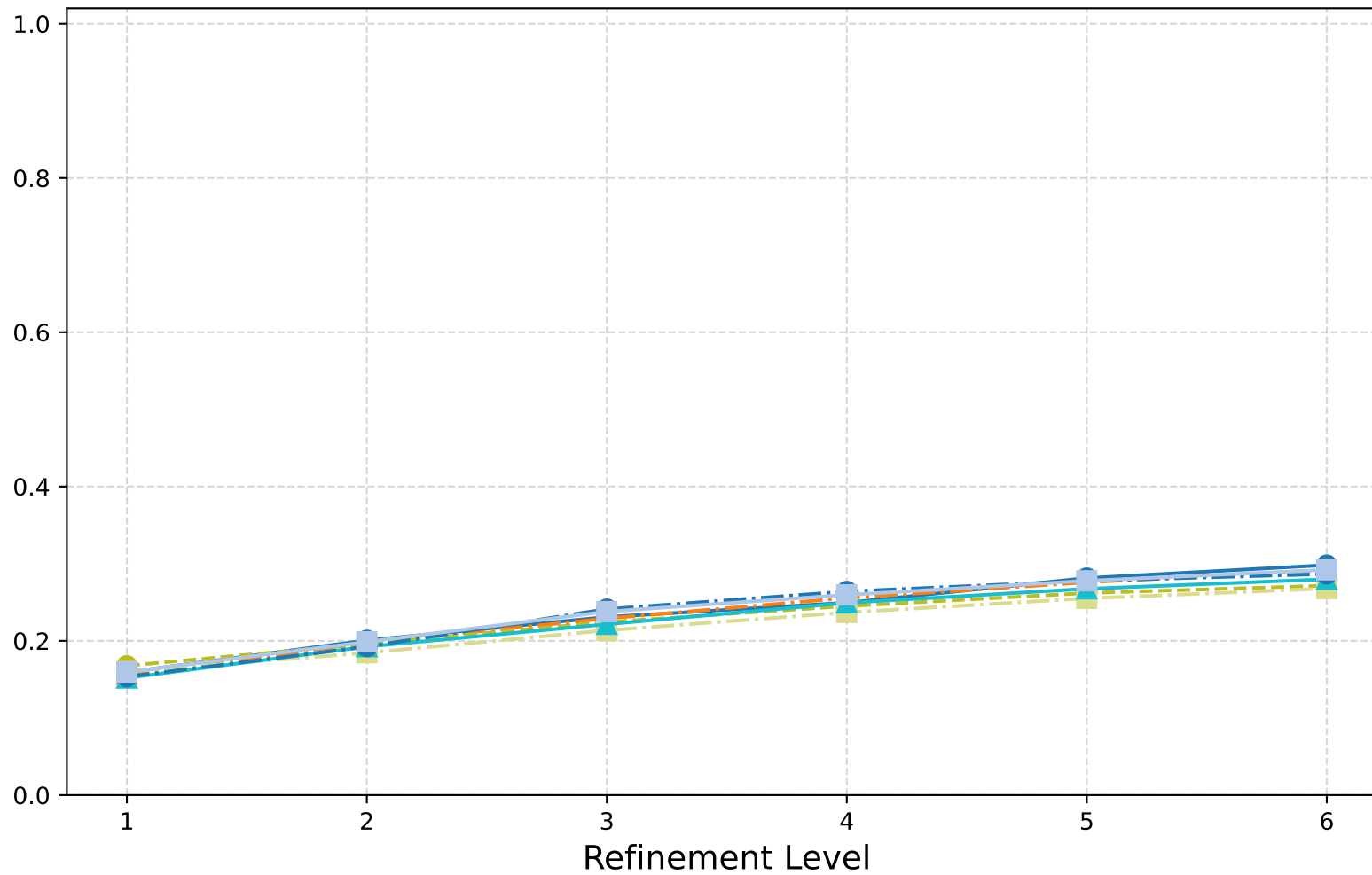
Magnetostatics: V-Cycle (Scaled Id) - n_{\text{ev}} -largest EV (mag.)
