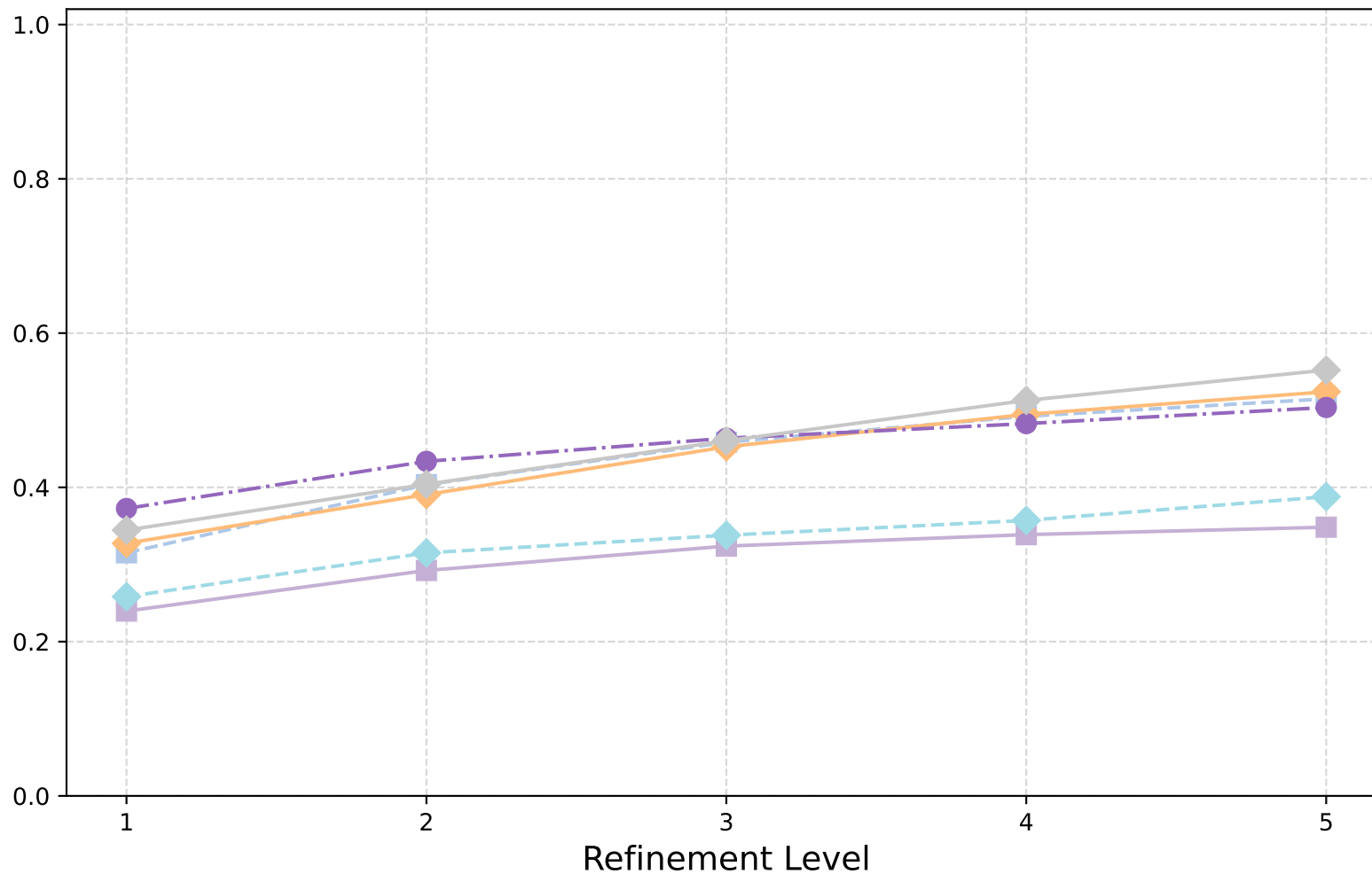
1-form Hodge Laplacian: V-Cycle (Scaled Id) - n_{\text{ev}} -largest EV (mag.)
