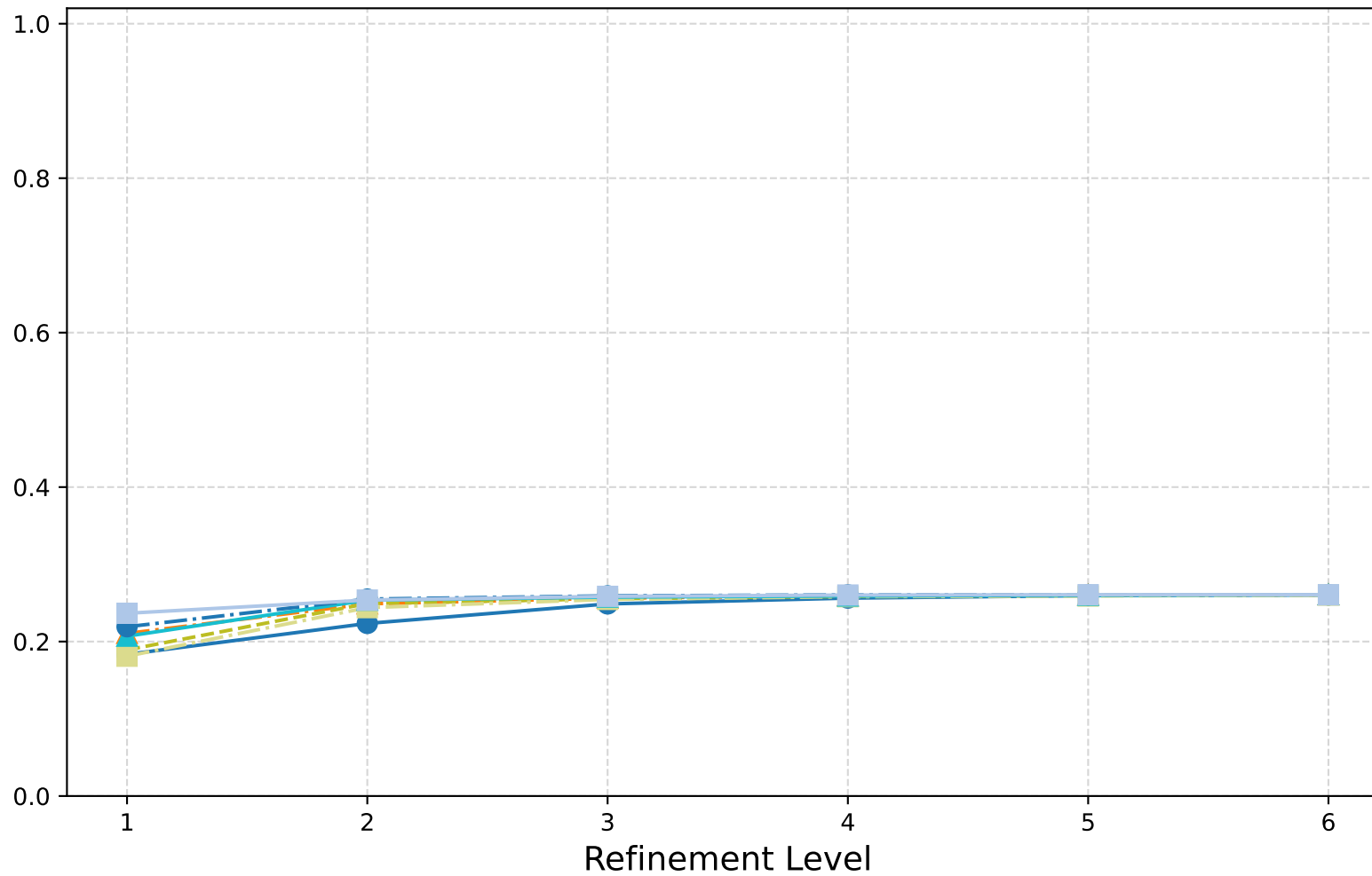
Dirac: W-Cycle (Scaled Id) - n_{\text{ev}} -largest EV (mag.)
