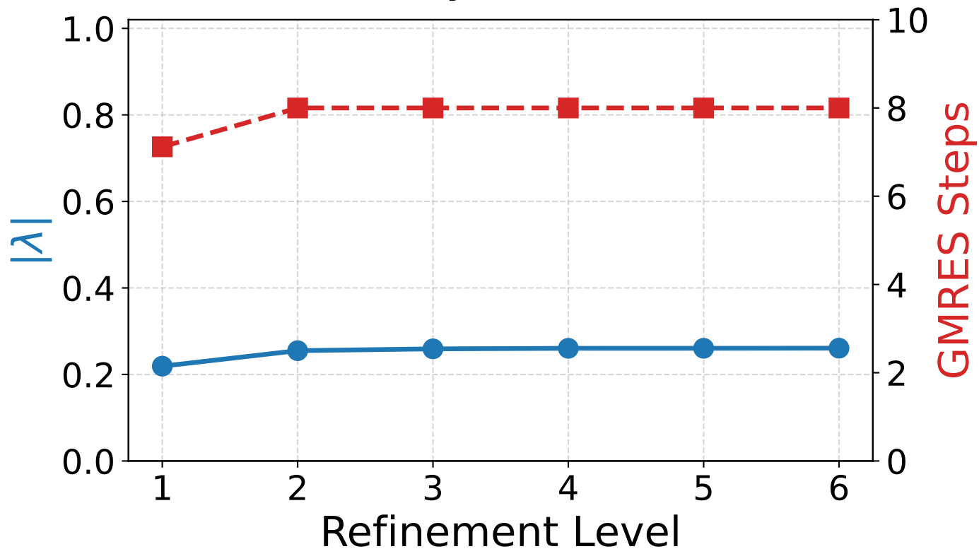
Dirac: W-Cycle (Scaled Id)
