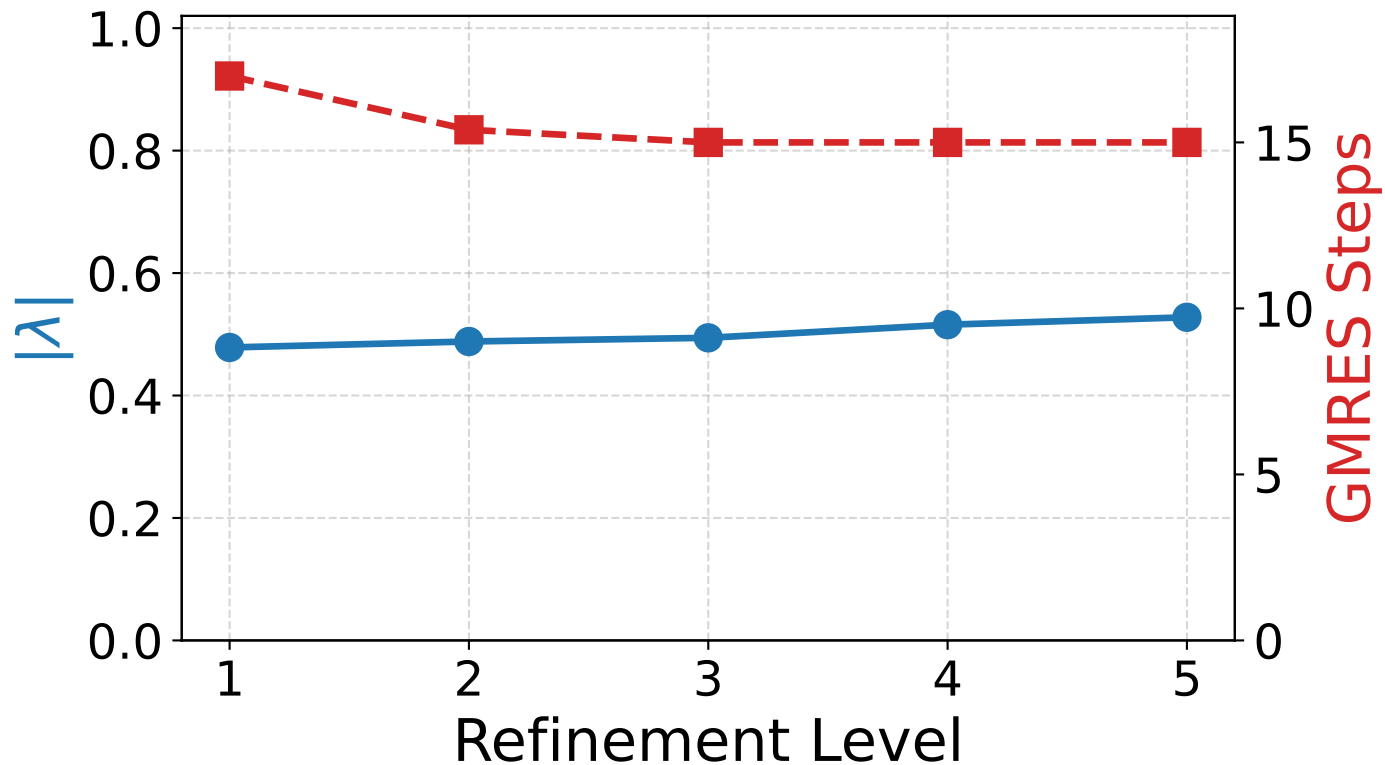
Dirac: W-Cycle (Scaled Id)
