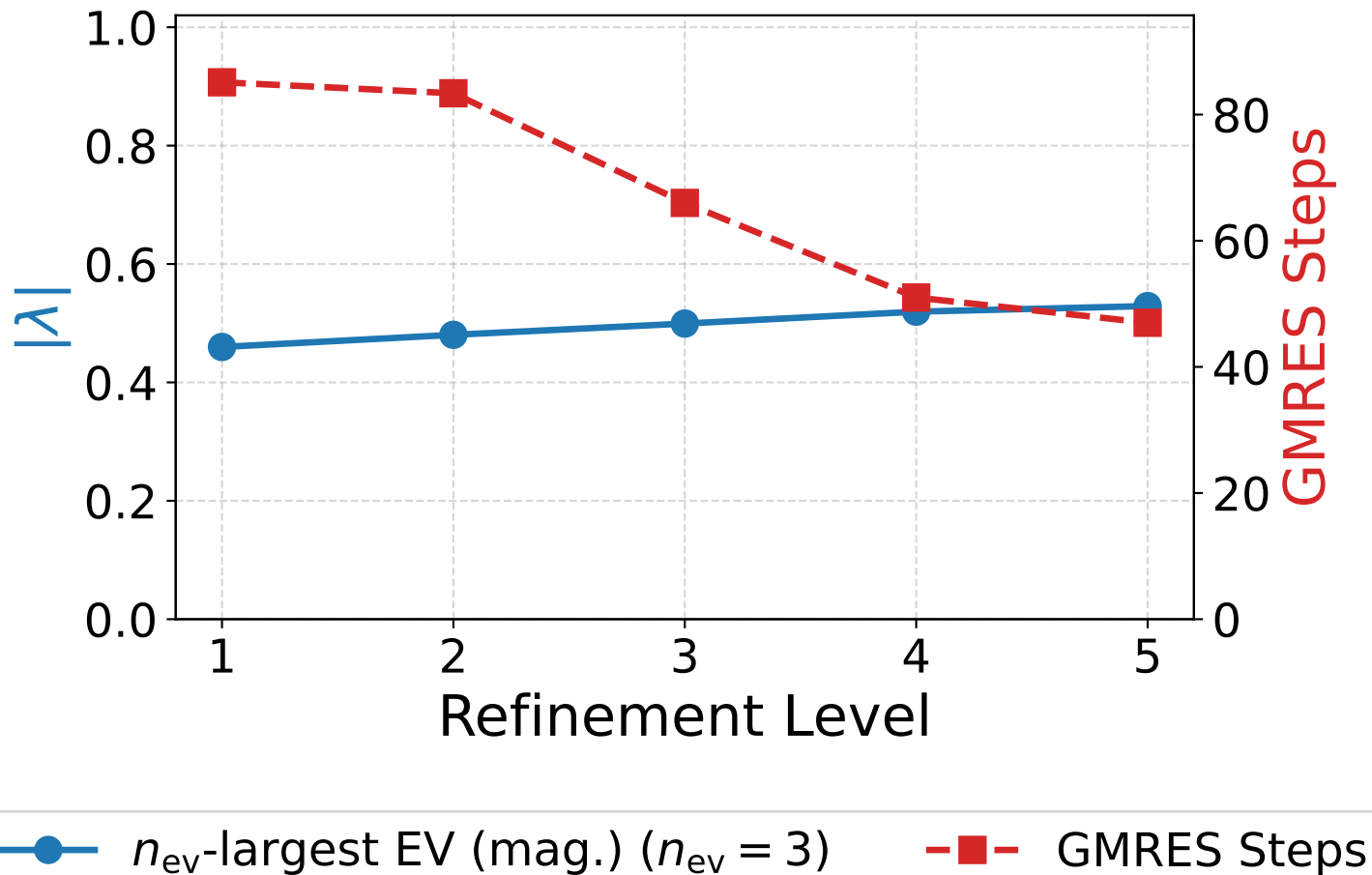
Dirac: W-Cycle (Scaled Id)
