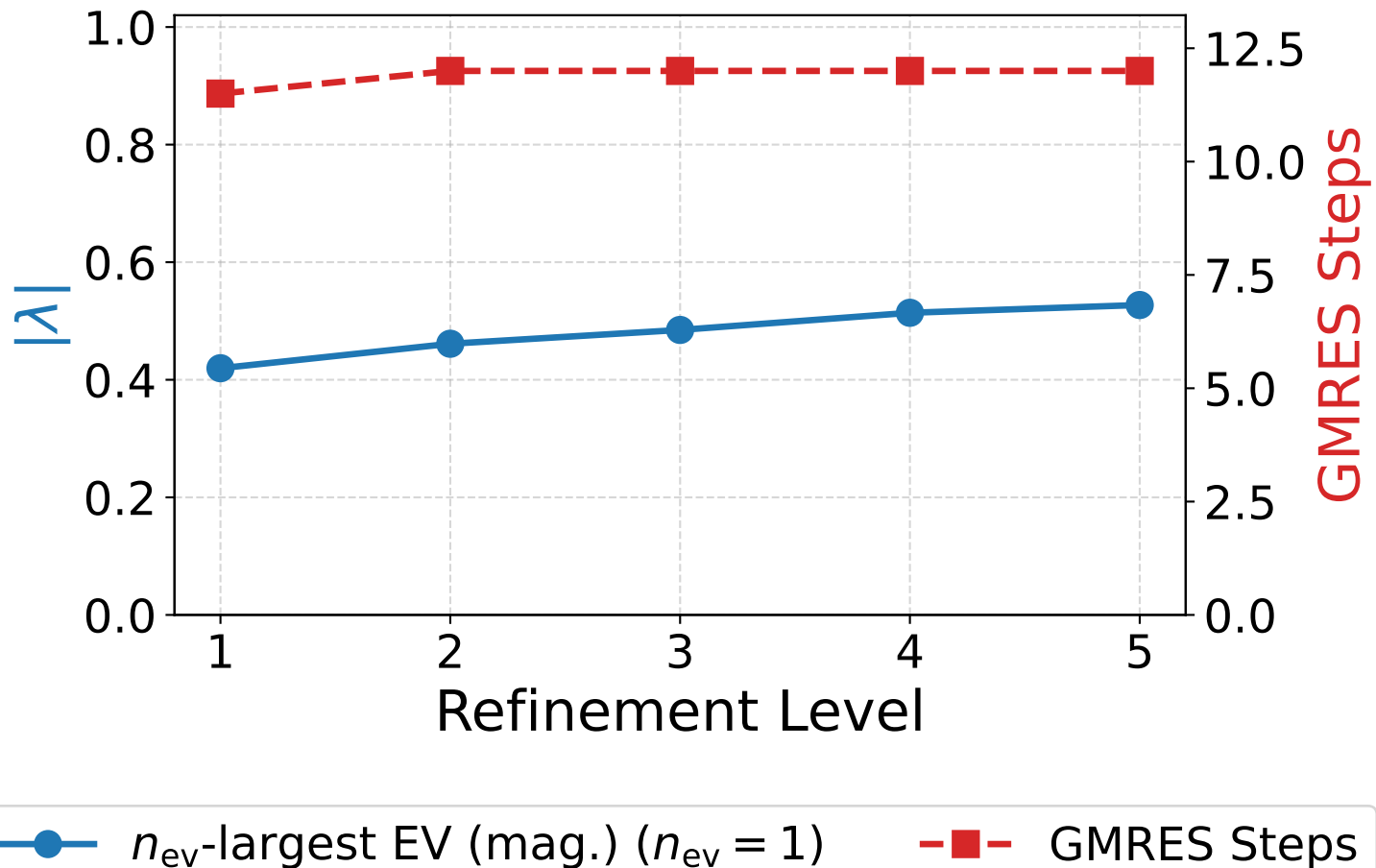
Dirac: W-Cycle (Scaled Id)
