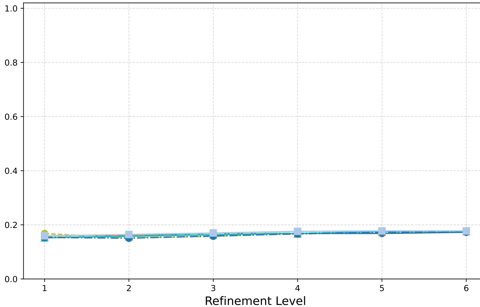
Magnetostatics: W-Cycle (Scaled Id) - n_{\text{ev}} -largest EV (mag.)
