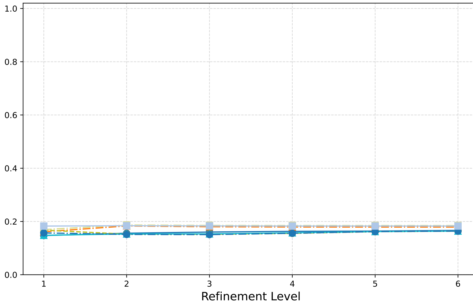
1-form Hodge Laplacian: W-Cycle (Scaled Id) - n_{\text{ev}} -largest EV (mag.)
