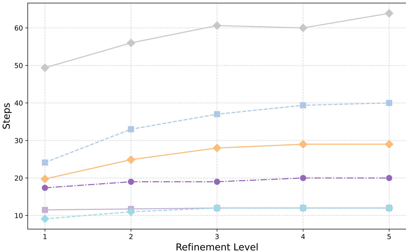
1-form Hodge Laplacian: W-Cycle (Scaled Id) - GMRES Iterations
