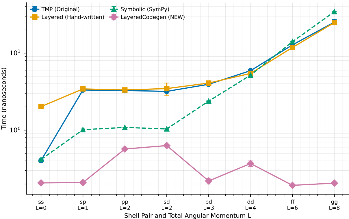
Hermite Expansion Coefficients: TMP vs Layered vs LayeredCodegen vs Symbolic
