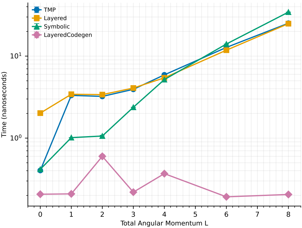
Hermite Coefficients: Scaling with Angular Momentum
