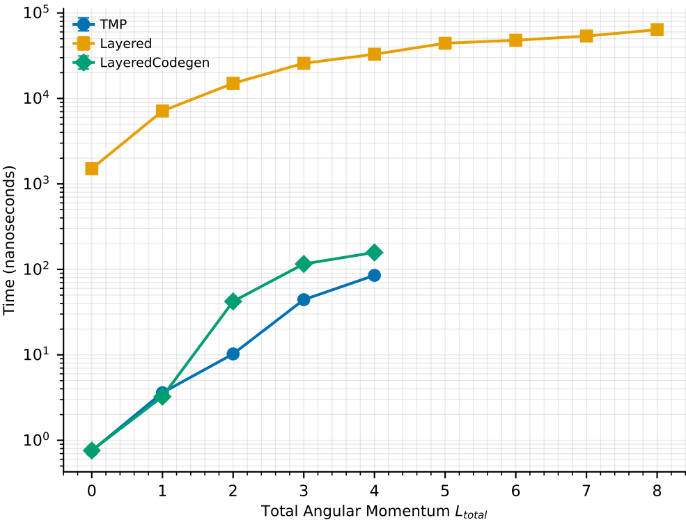
Coulomb Hermite Integrals: TMP vs Layered vs LayeredCodegen
