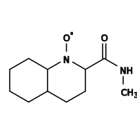
MULMUC
