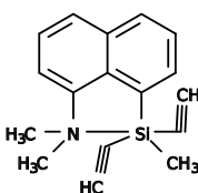
FAPWEZ
