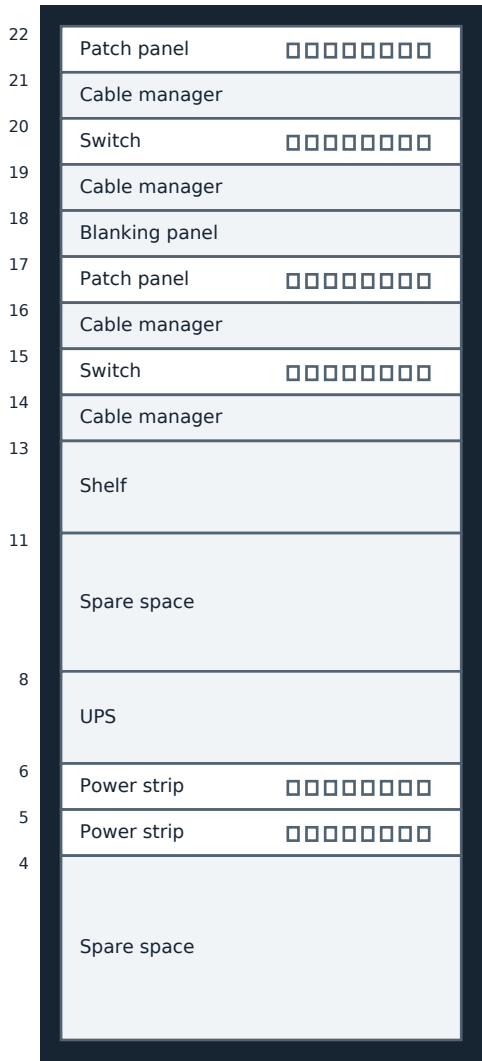
Front view · 22U
