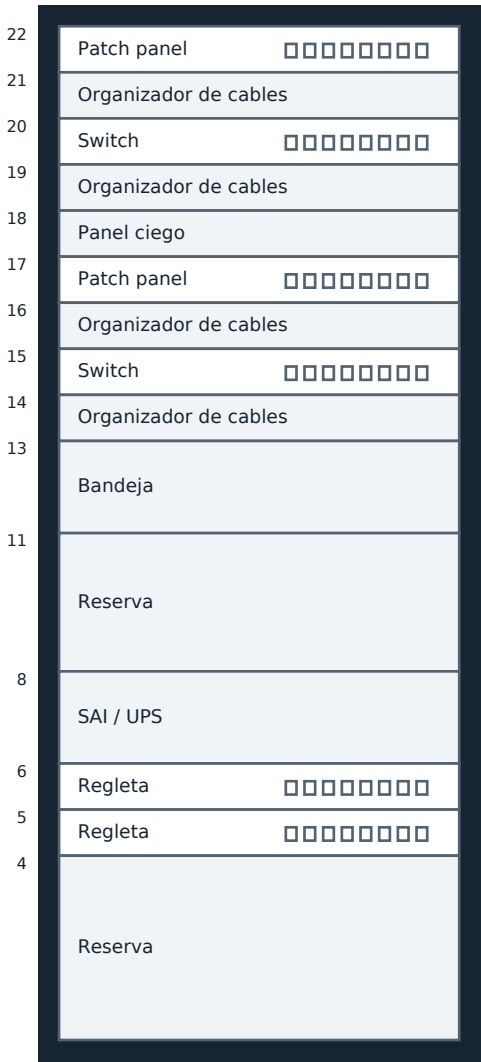
Vista frontal - 22U
