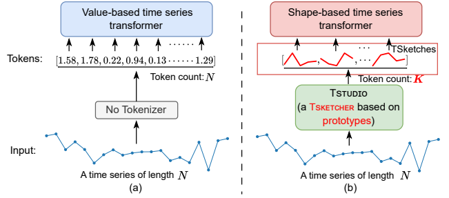
Fig. 2. (a) Value-based time series transformer, e.g., [17]. (b) Time series transformer with TSketches obtained from TSTUDIO.
