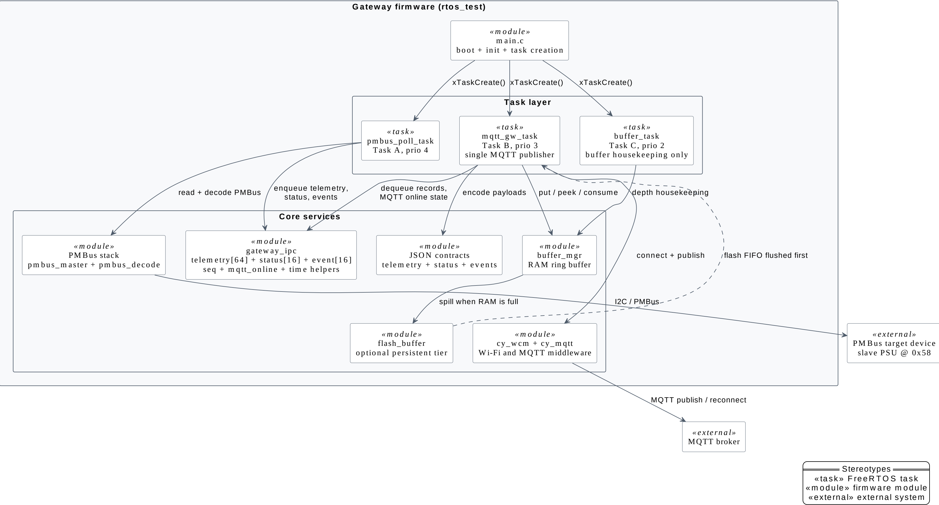
Figure 2.1. UML component view of FreeRTOS tasks and IPC
