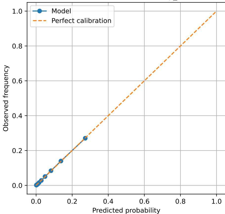
Calibration curve: coronary_hd
