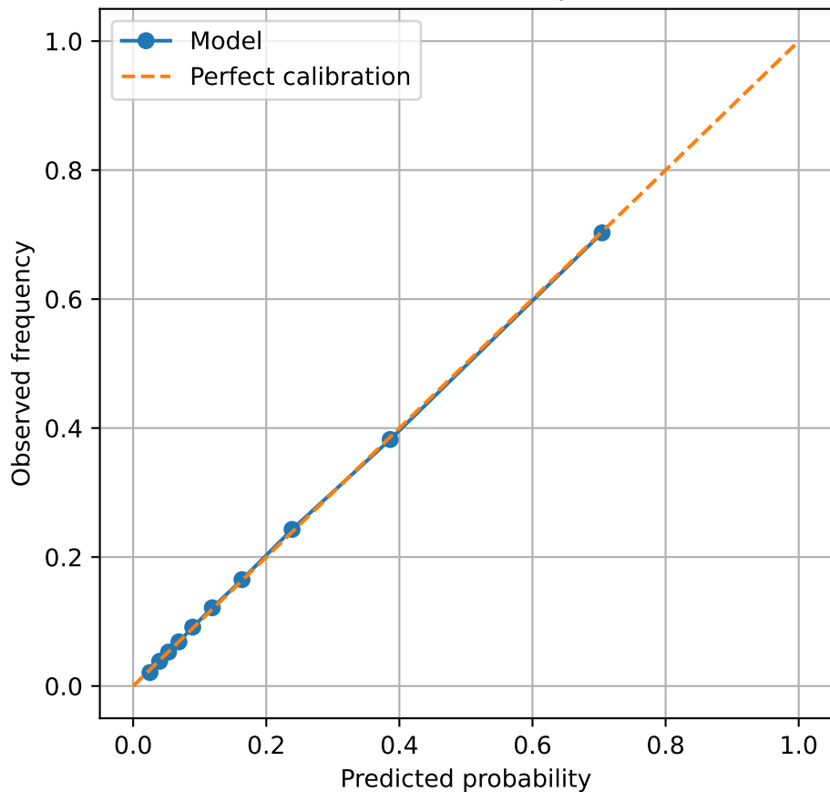
Calibration curve: depression
