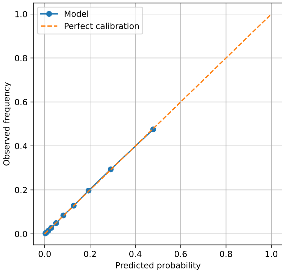
Calibration curve: diabetes
