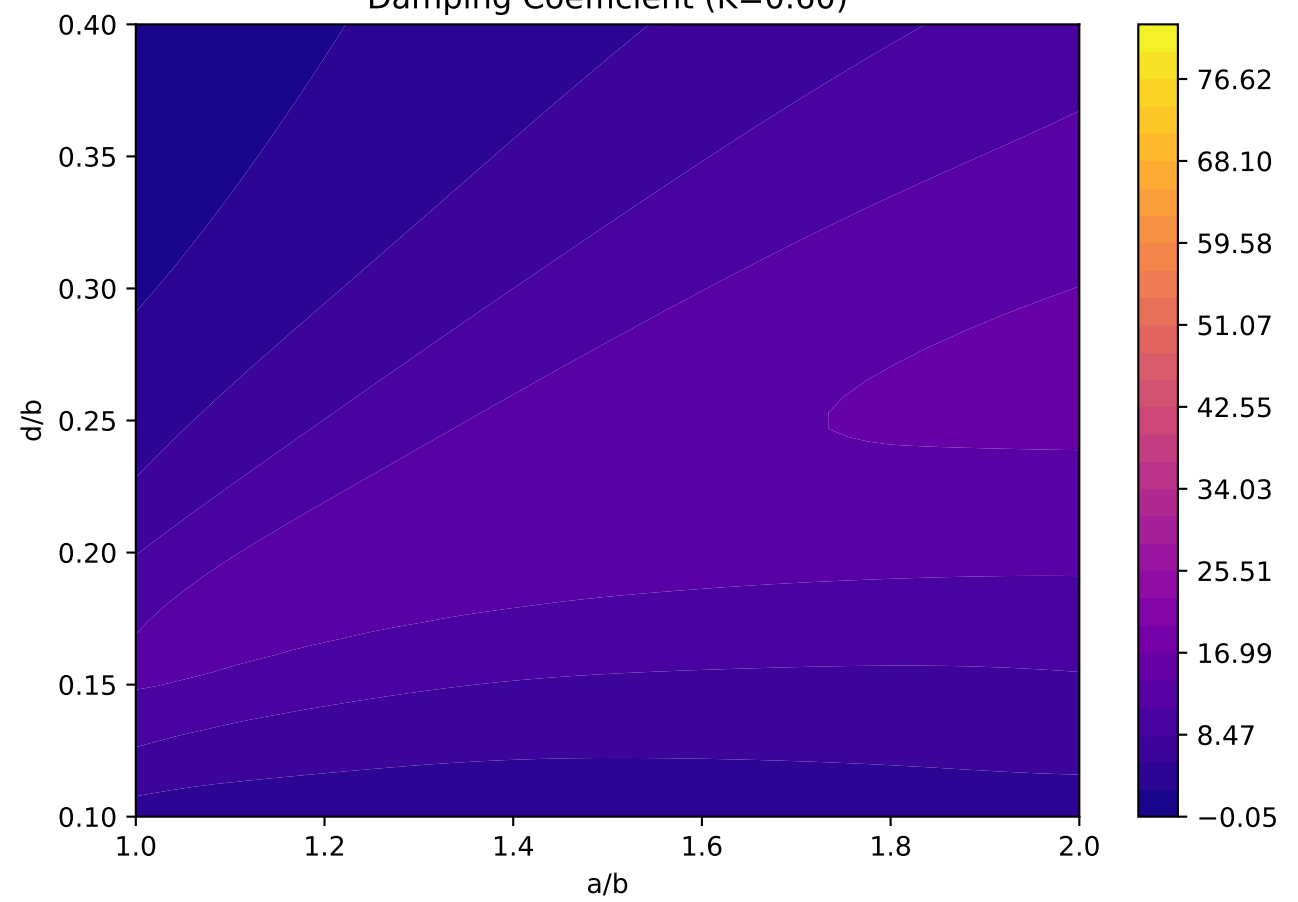
Damping Coefficient (K=0.60)
