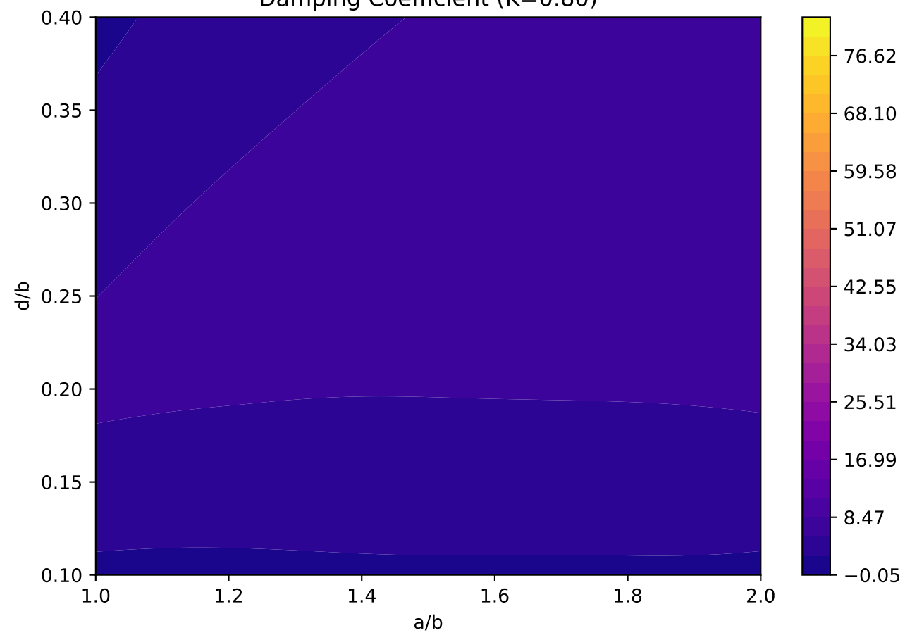
Damping Coefficient (K=0.80)
