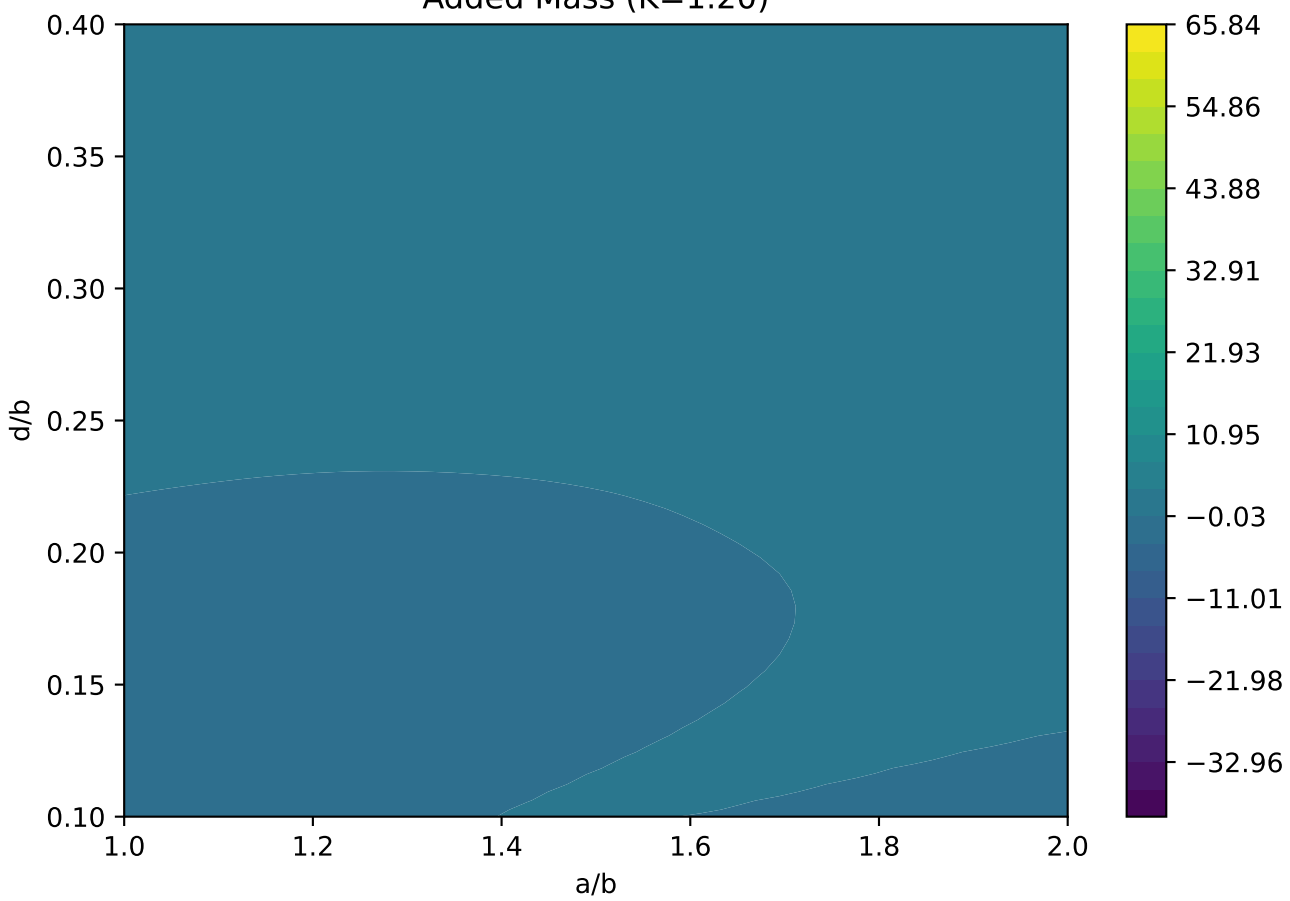
Added Mass (K=1.20)
