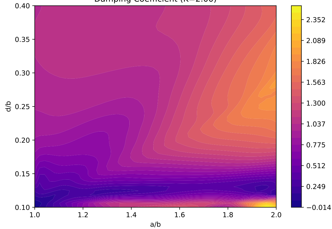
Damping Coefficient (K=2.00)
