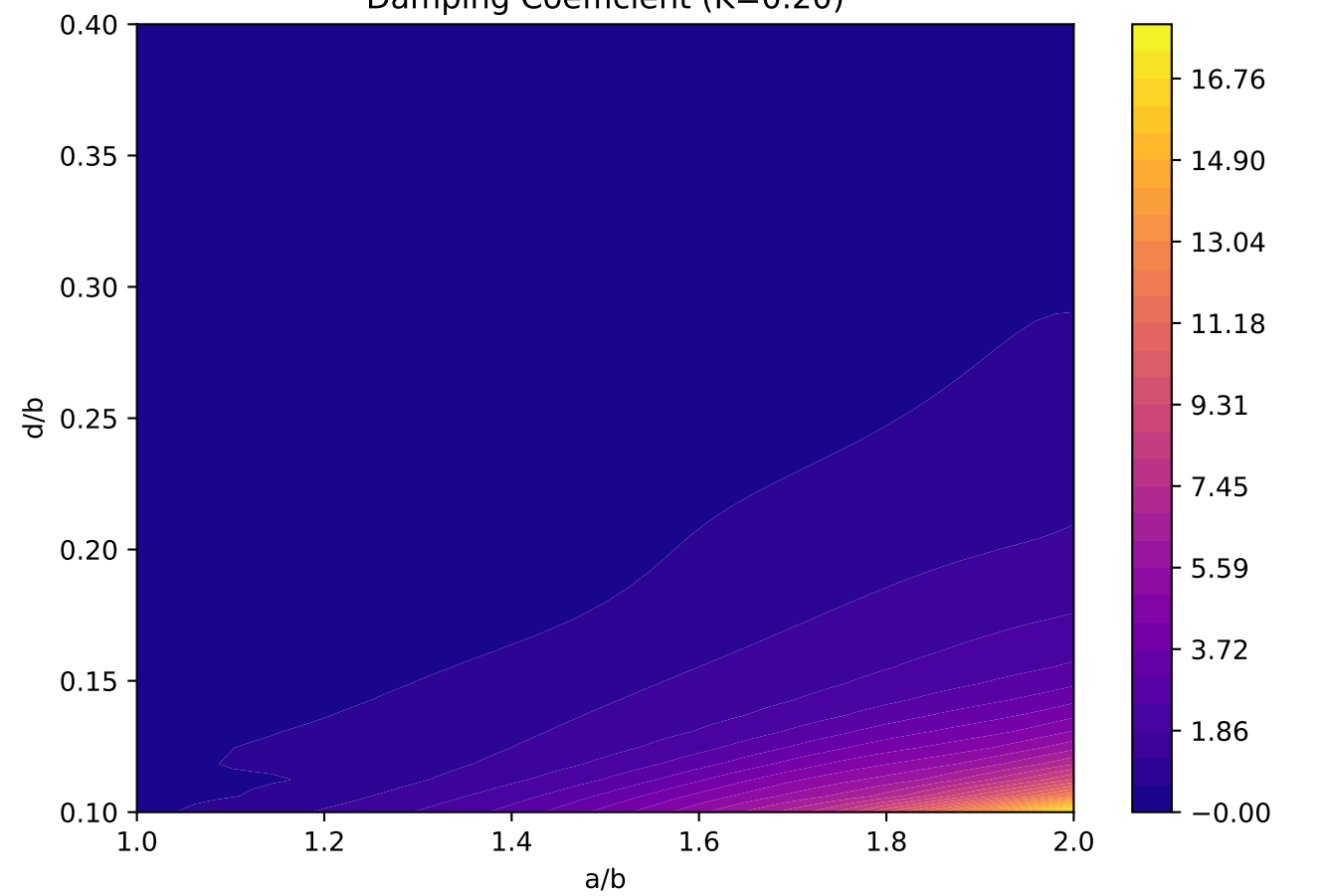
Damping Coefficient ( K=0.20 )
