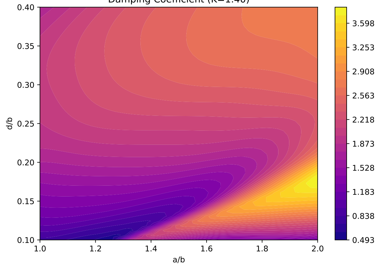
Damping Coefficient (K=1.40)
