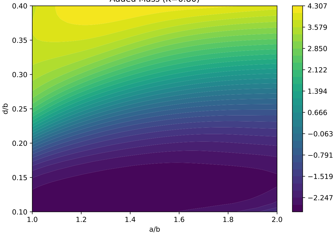
Added Mass (K=0.80)
