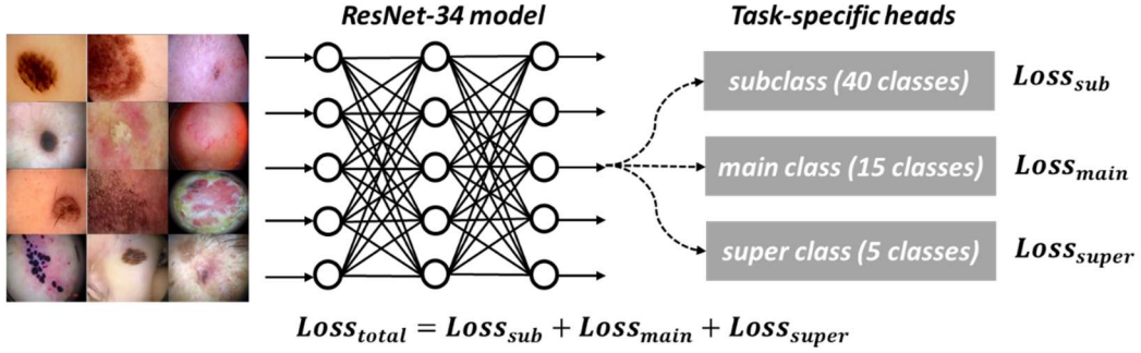
Figure 1. Illustration of the multi-task approach for hierarchical skin lesion classification.
