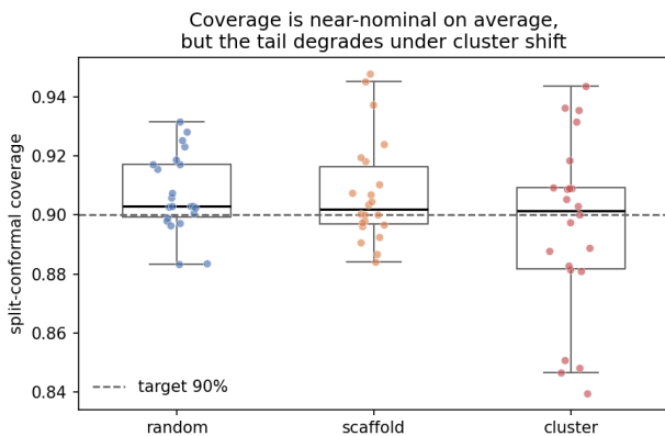
Figure 4: Split-conformal coverage per endpoint (target 0.90). Near-nominal on average for all splits, but the lower tail degrades under cluster shift (worst: BBB \approx 0.84 ); degradation is endpoint-specific, not uniform.
