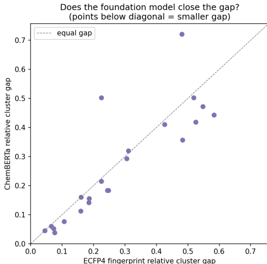
Figure 4: ChemBERTa vs. ECFP4 relative cluster gap. Points below the diagonal = smaller gap.
