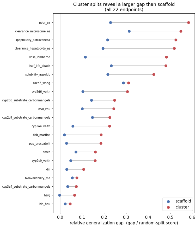
Figure 1: Relative generalization gap per endpoint: cluster (red) exceeds scaffold (blue) on all 22 endpoints. hERG, flat under scaffold, shows a positive cluster gap.
