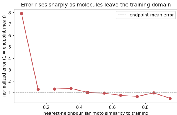
Figure 2: Normalized error vs. nearest-neighbour similarity to training (mean over 22 endpoints).
