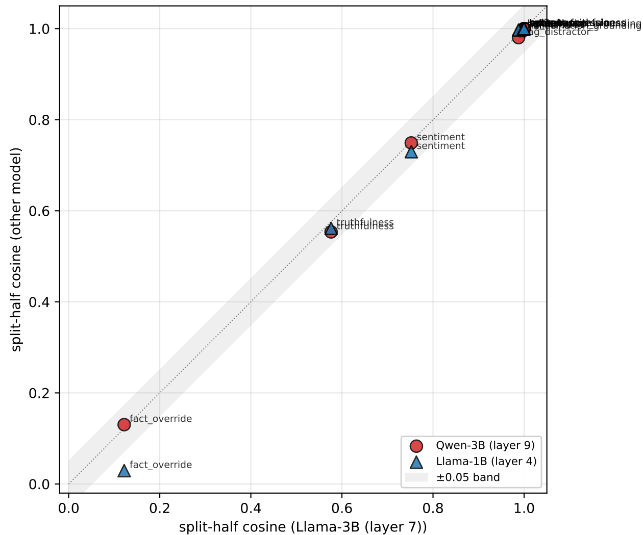
Cross-model agreement: geometric features depend on the contrast, not the model
