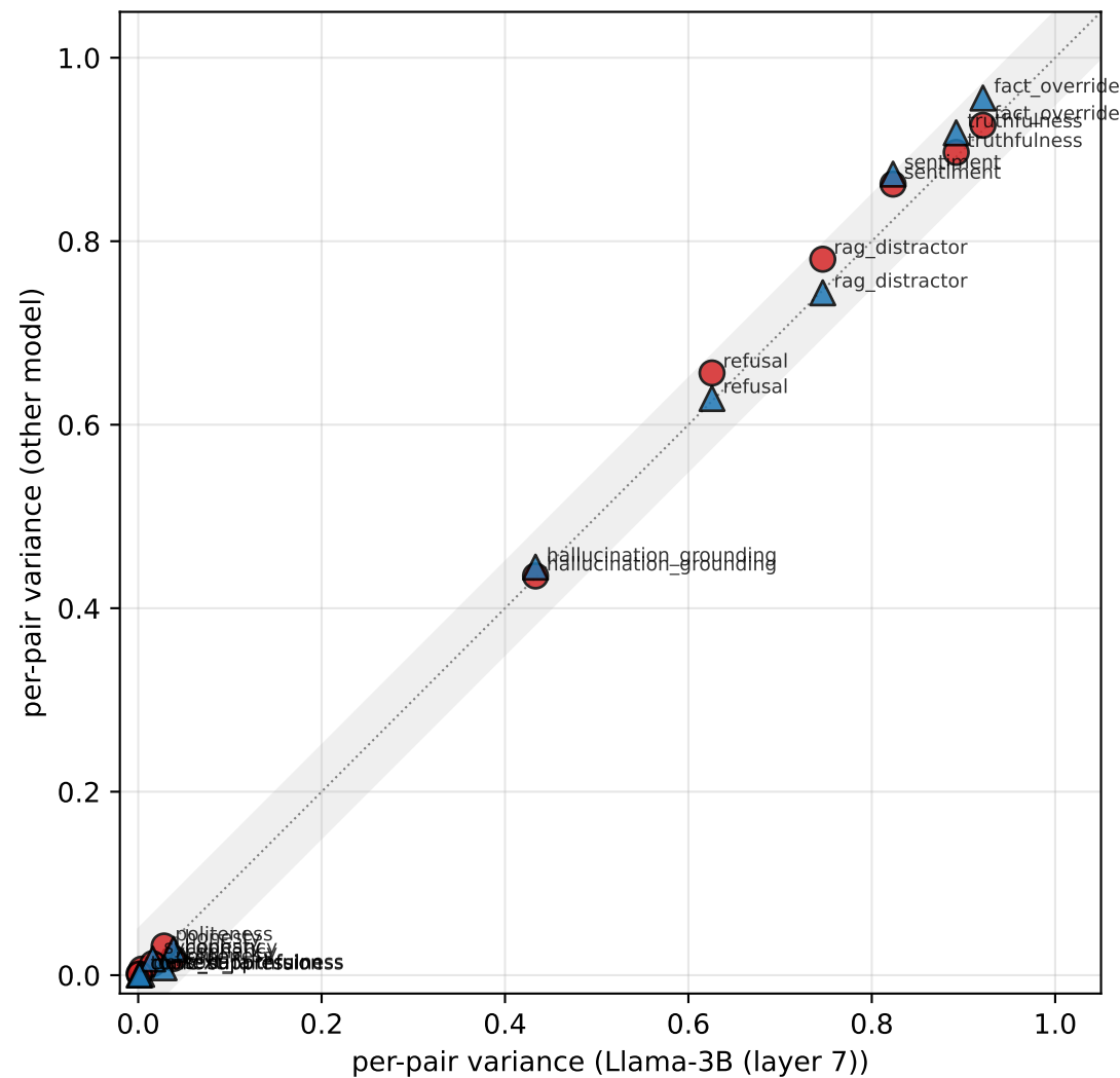
Cross-model agreement: geometric features depend on the contrast, not the model
